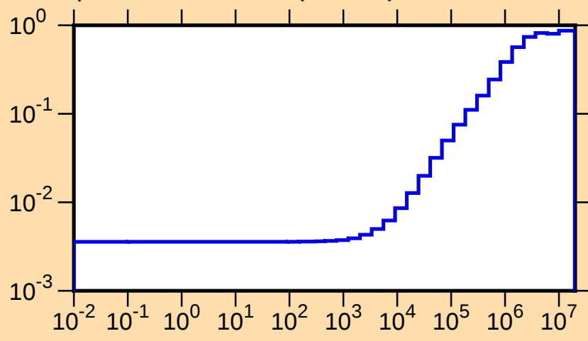
\mu vs. E for ^{190}\text{Os}(\text{mt251})
