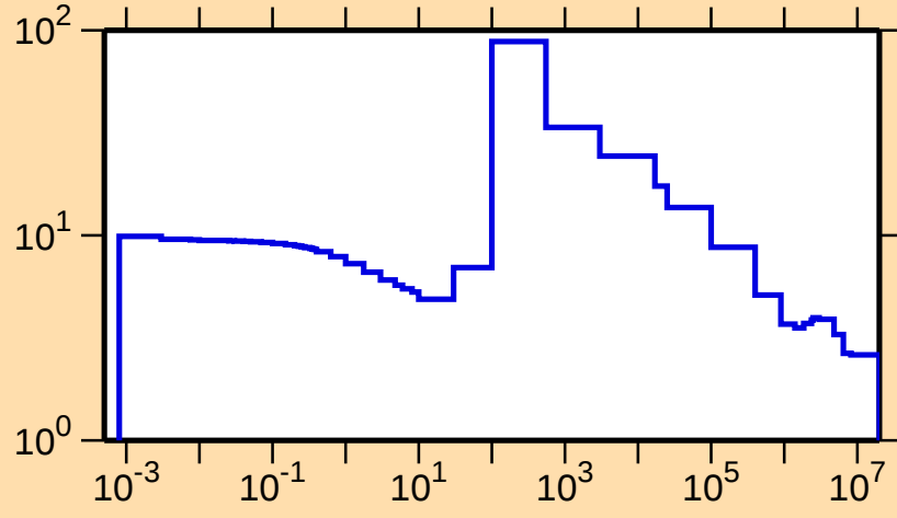
\sigma vs. E for ^{190}\text{Os}(n,\text{el.})
