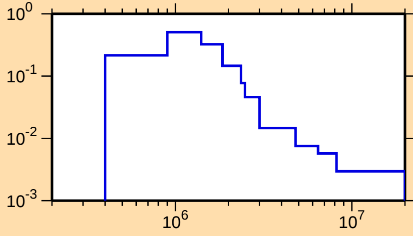
\sigma vs. E for ^{190}\text{Os}(n,n_3)
