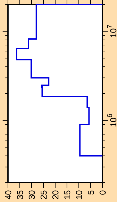
\Delta\sigma/\sigma vs. E for ^{190}\text{Os}(n,n_3)
