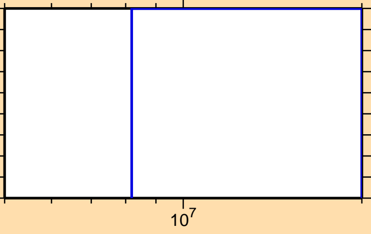
\sigma vs. E for ^{190}\text{Os}(n,\text{nd})
