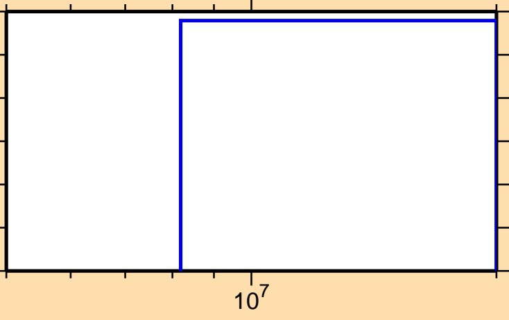
\sigma vs. E for ^{190}\text{Os}(n,t)
