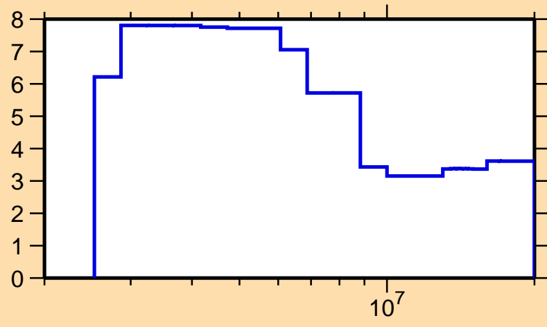
\Delta\sigma/\sigma vs. E for ^{191}\text{Os}(n,\text{tot.})
