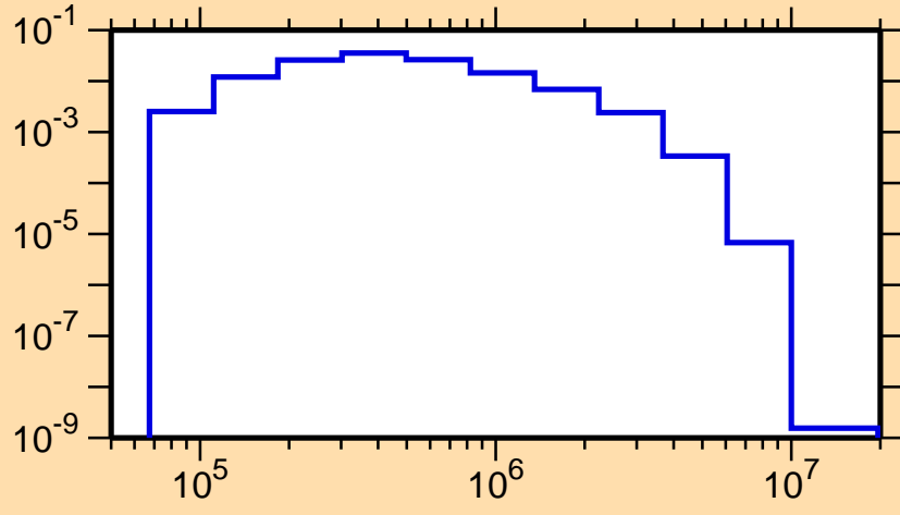
\sigma vs. E for ^{191}\text{Os}(n,n_1)
