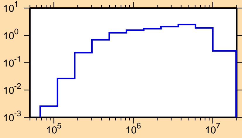
\sigma vs. E for ^{191}\text{Os}(n,\text{inel.})
