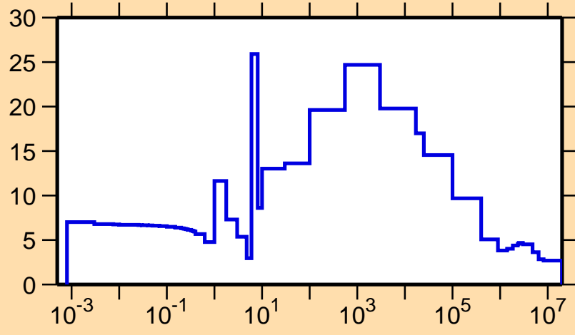
\sigma vs. E for ^{191}\text{Os}(n,\text{el.})
