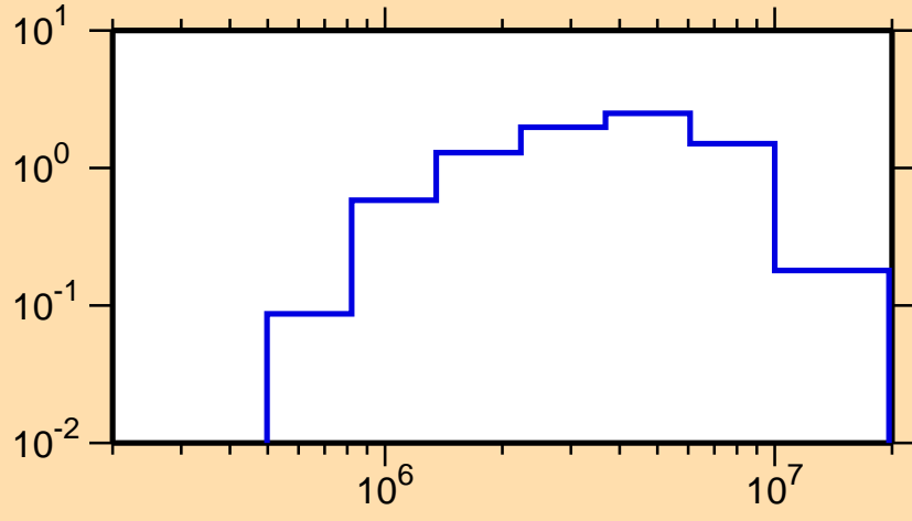
\sigma vs. E for ^{191}\text{Os}(n,n\text{cont.})
