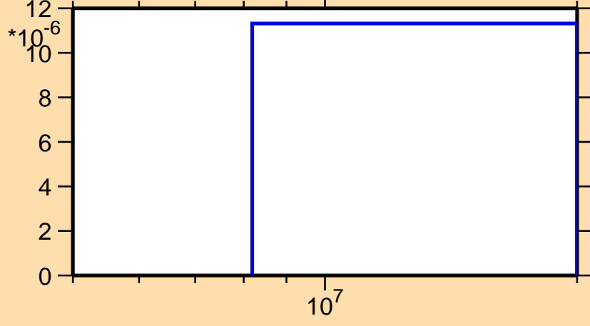
\sigma vs. E for ^{191}\text{Os}(n,t)
