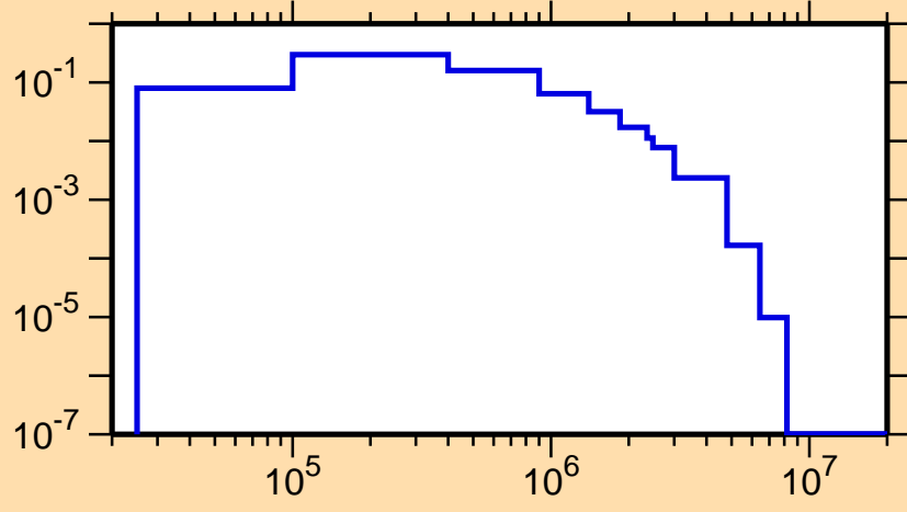
\sigma vs. E for ^{191}\text{Os}(n,n_3)
