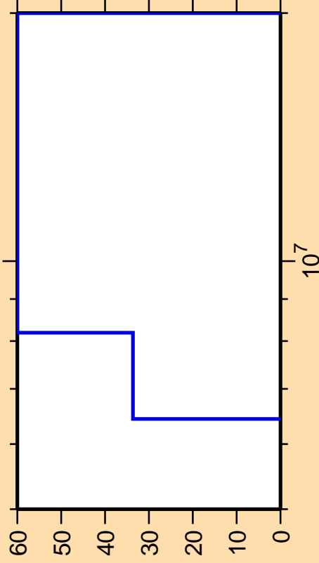
\Delta\sigma/\sigma vs. E for ^{191}\text{Os}(n,n\alpha)
