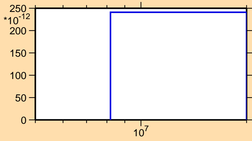
\sigma vs. E for ^{191}\text{Os}(n,nt)
