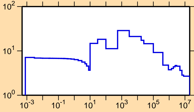
\sigma vs. E for ^{191}\text{Os}(n,\text{el.})
