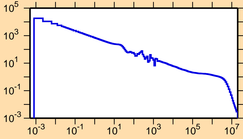
\sigma vs. E for ^{192}\text{Os}(n,\gamma)
