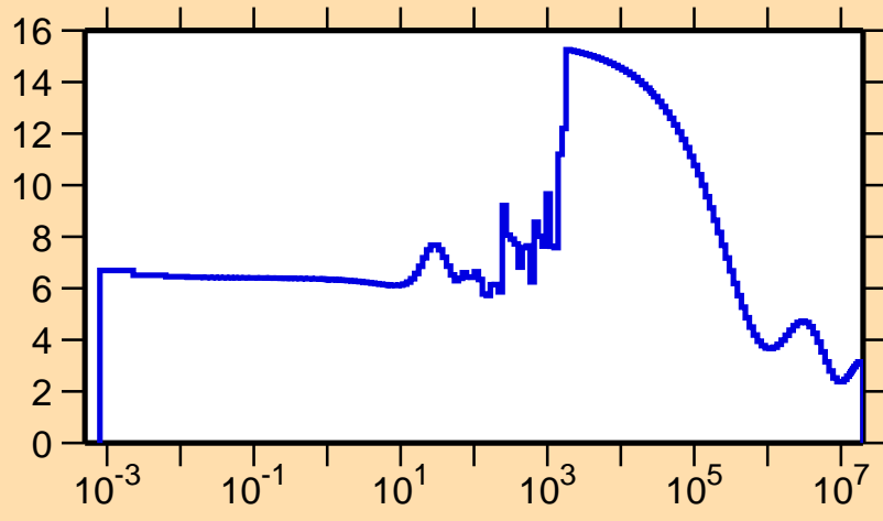
\sigma vs. E for ^{192}\text{Os}(n,\text{el.})
