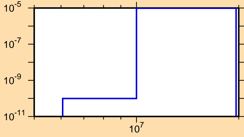
\sigma vs. E for ^{192}\text{Os}(n,n\alpha)
