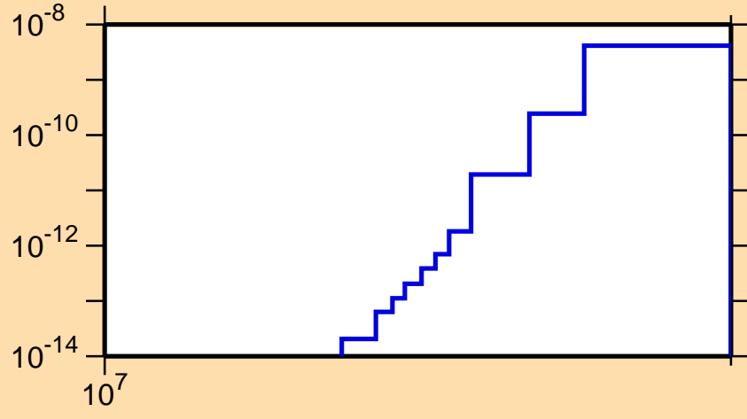
\sigma vs. E for ^{193}\text{Os}(n,2n\alpha)
