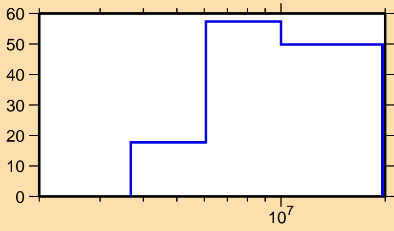
\Delta\sigma/\sigma vs. E for ^{193}\text{Os}(n,p)
