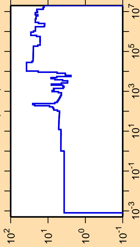
\Delta\sigma/\sigma vs. E for ^{194}\text{Os}(n,\text{el.})
