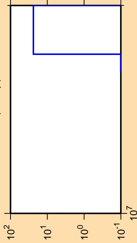
\Delta\sigma/\sigma vs. E for ^{194}\text{Os}(n,2np)
