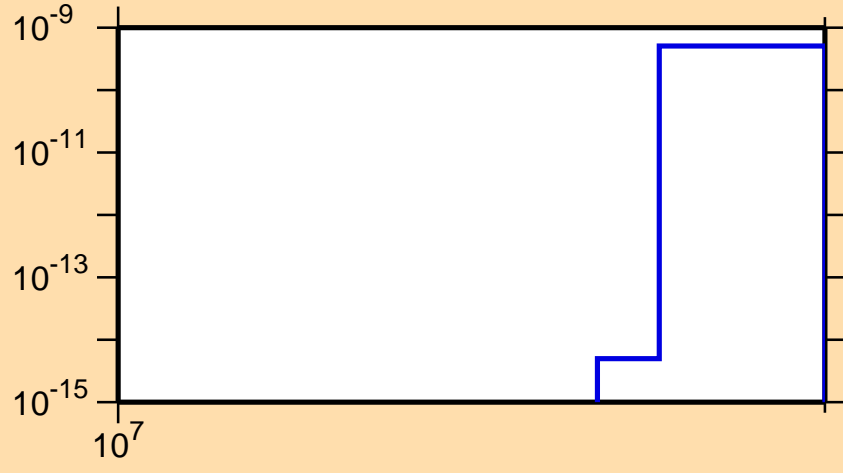
\sigma vs. E for ^{194}\text{Os}(n,\text{nd})
