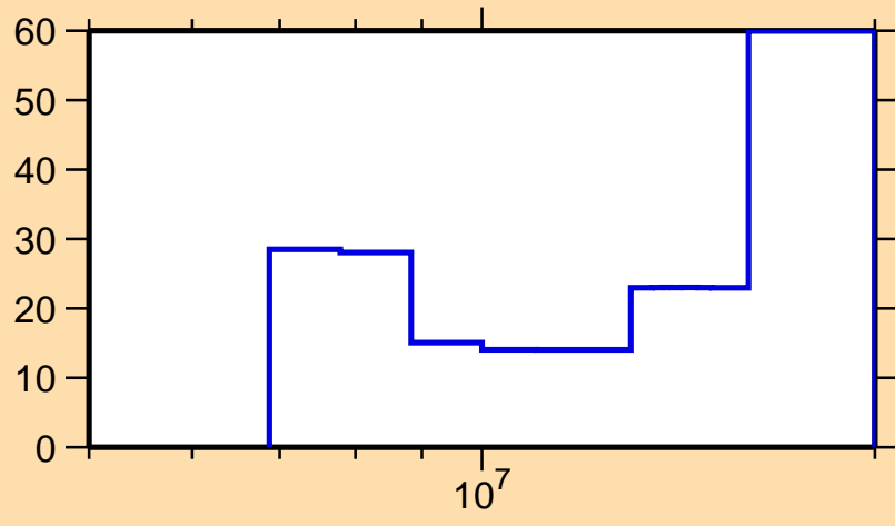
\Delta\sigma/\sigma vs. E for ^{194}\text{Os}(n,2n)
