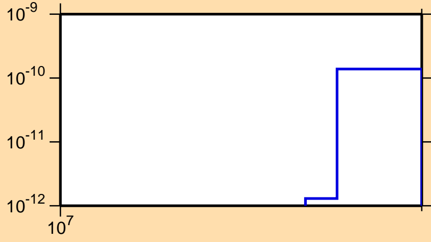
\sigma vs. E for ^{194}\text{Os}(n,2n\alpha)
