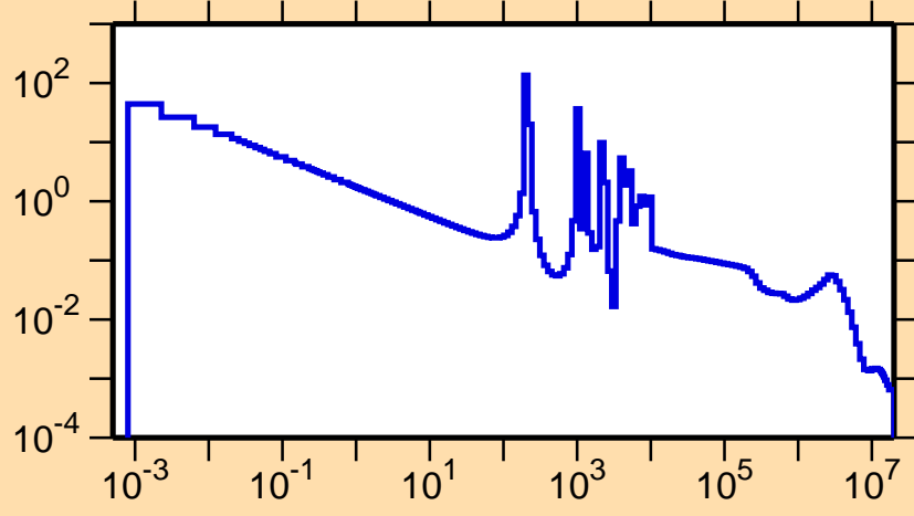
\sigma vs. E for ^{194}\text{Os}(n,\gamma)
