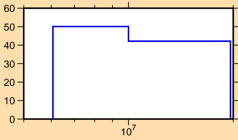
\Delta\sigma/\sigma vs. E for ^{194}\text{Os}(n,n_1)
