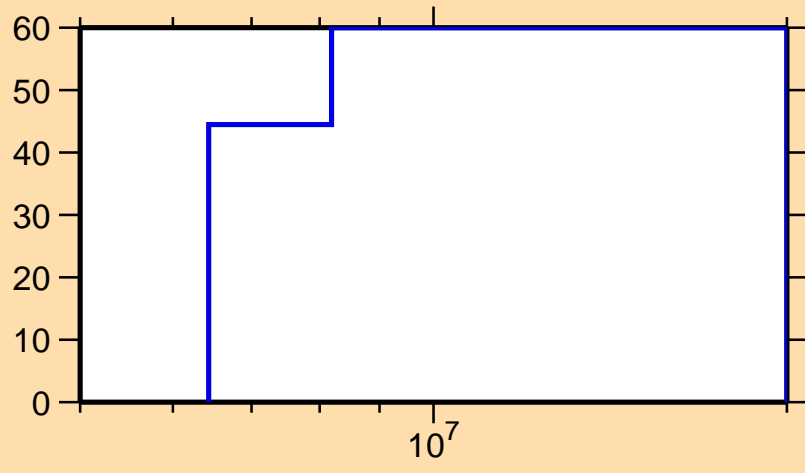
\Delta\sigma/\sigma vs. E for ^{194}\text{Os}(n,p)
