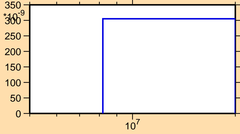
\sigma vs. E for ^{195}\text{Os}(n,n\alpha)
