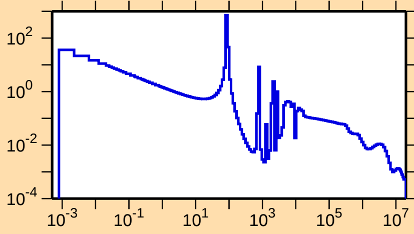
\sigma vs. E for ^{196}\text{Os}(n,\gamma)
