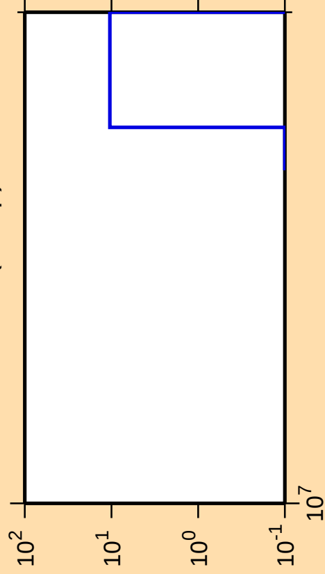
\Delta\sigma/\sigma vs. E for ^{196}\text{Os}(n,2np)
