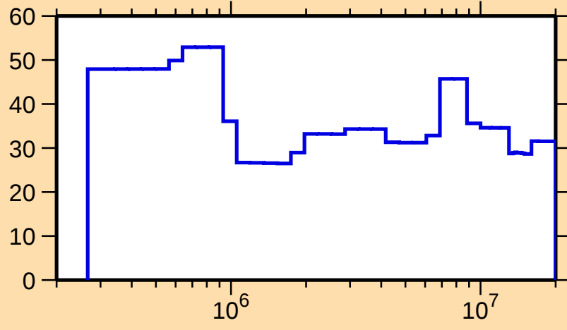
\Delta\sigma/\sigma vs. E for ^{196}\text{Os}(n,\text{el.})
