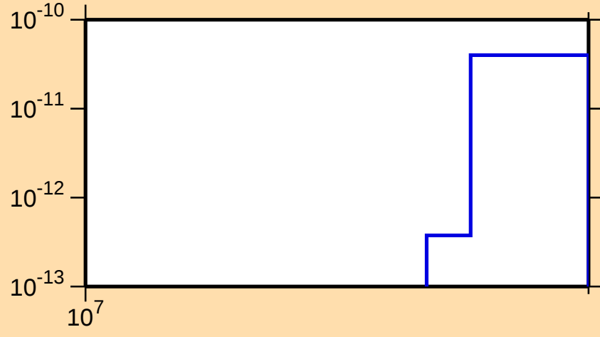
\sigma vs. E for ^{196}\text{Os}(n,2n\alpha)
