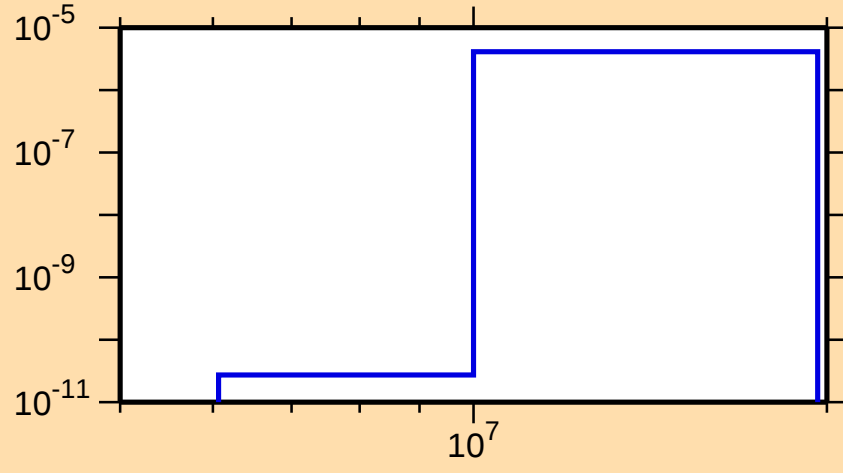
\sigma vs. E for ^{196}\text{Os}(n,\alpha)
