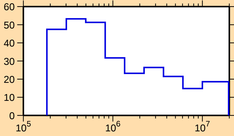
\Delta\sigma/\sigma vs. E for ^{196}\text{Os}(n,\text{tot.})
