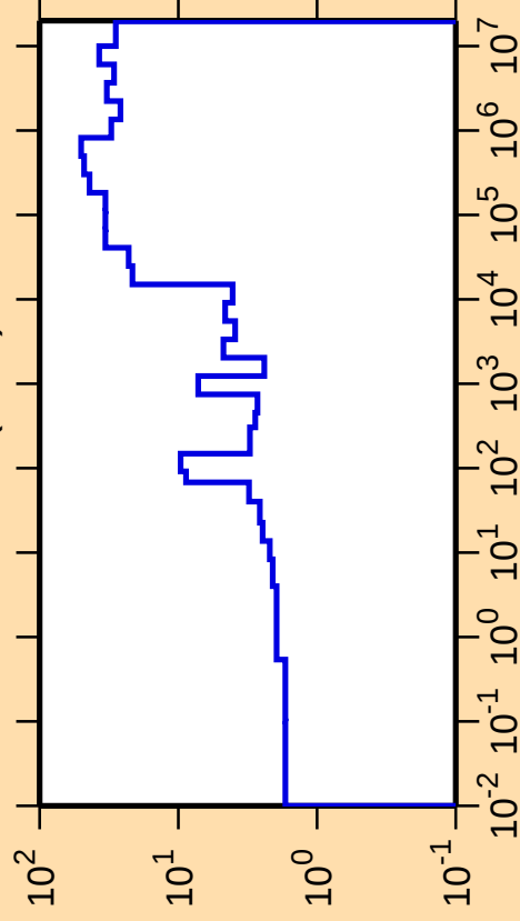
\Delta\sigma/\sigma vs. E for ^{196}\text{Os}(n,\text{el.})
