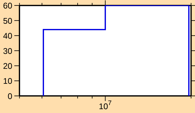
\Delta\sigma/\sigma vs. E for ^{196}\text{Os}(n,n\text{cont.})
