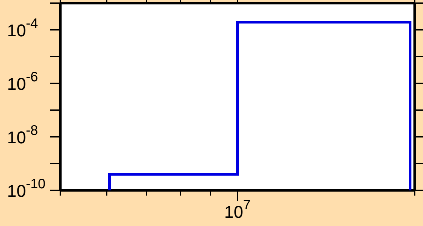
\sigma vs. E for ^{196}\text{Os}(n,p)
