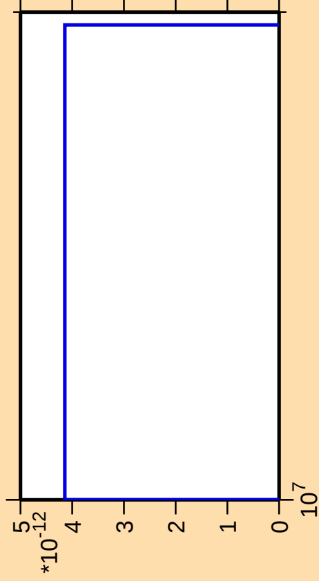
\Delta\sigma/\sigma vs. E for ^{196}\text{Os} (mt 11)
