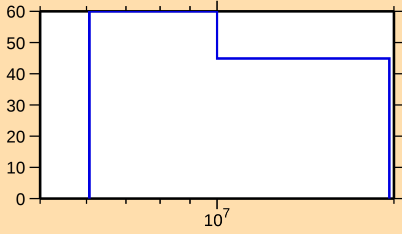
\Delta\sigma/\sigma vs. E for ^{196}\text{Os}(n,2n)
