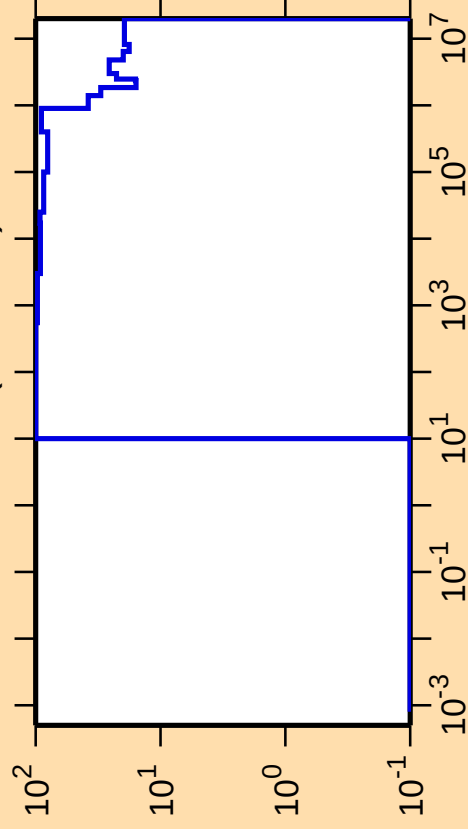
\Delta\sigma/\sigma vs. E for ^{196}\text{Os}(n,\text{nonel.})
