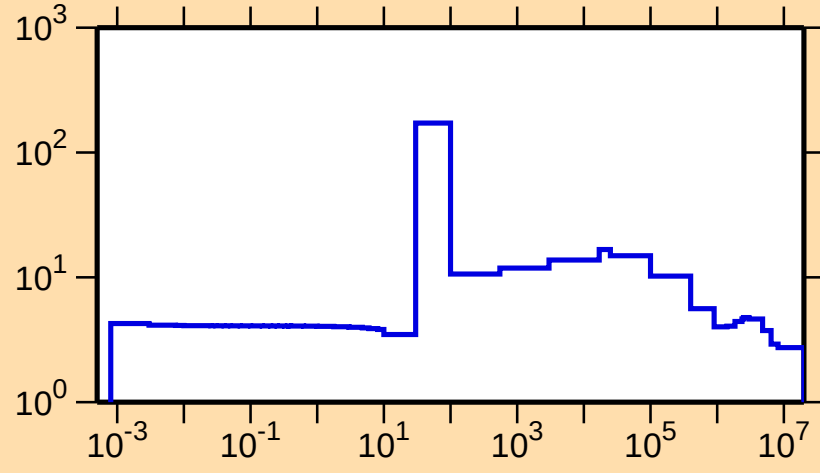
\sigma vs. E for ^{196}\text{Os}(n,\text{el.})
