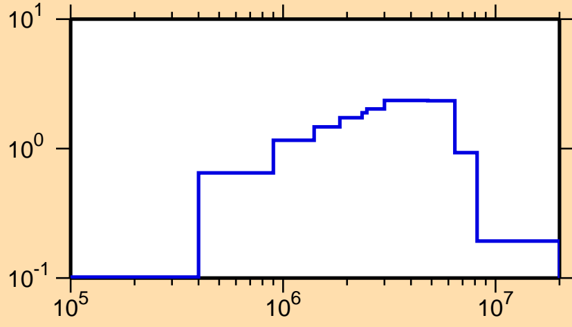
\sigma vs. E for ^{197}\text{Os}(n,n\text{cont.})
