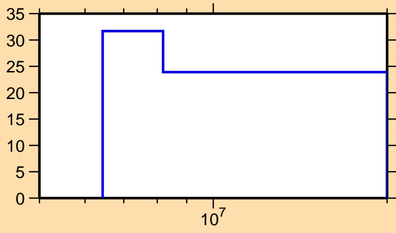
\Delta\sigma/\sigma vs. E for ^{197}\text{Os}(n,ncont.)
