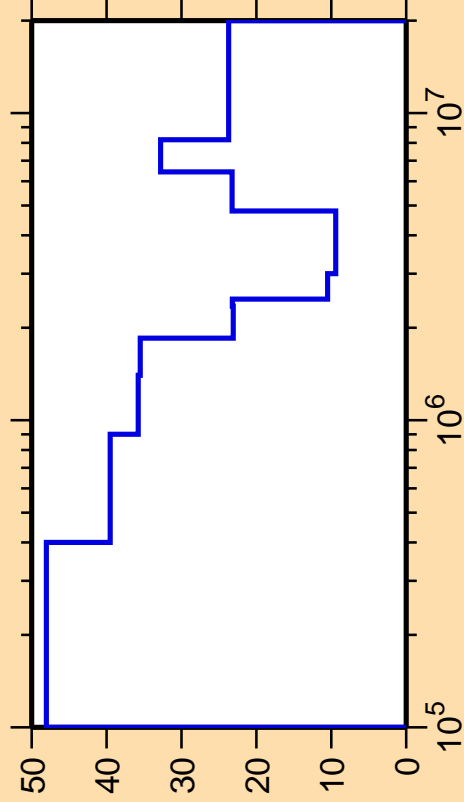
\Delta\sigma/\sigma vs. E for ^{197}\text{Os}(n,\text{inel.})
