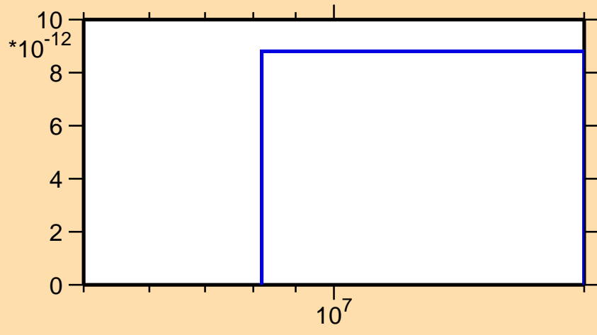
\sigma vs. E for ^{197}\text{Os}(n,2np)
