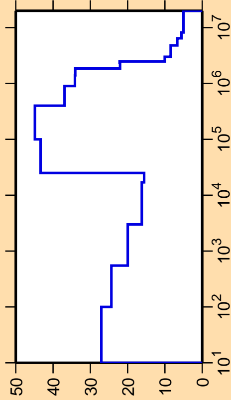
\Delta\sigma/\sigma vs. E for ^{197}\text{Os}(n,\text{nonel.})
