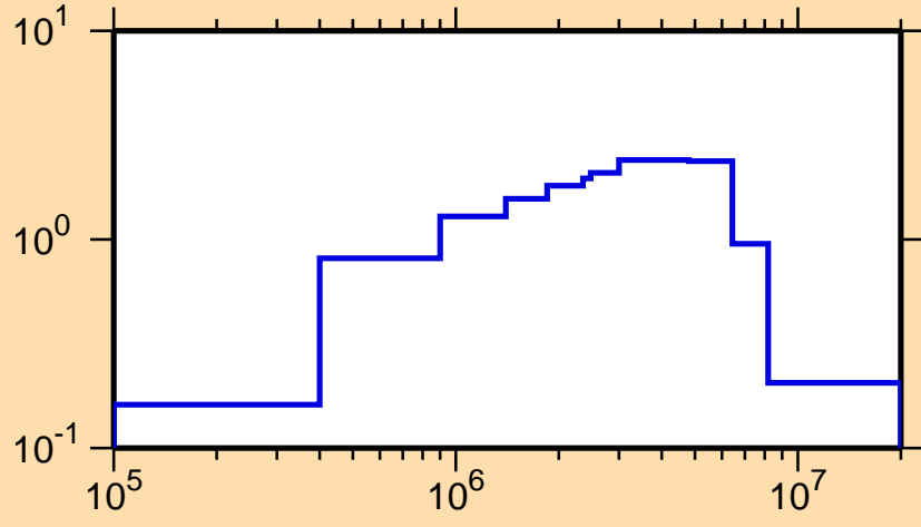
\sigma vs. E for ^{197}\text{Os}(n,\text{inel.})
