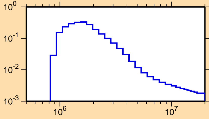
\sigma vs. E for ^{198}\text{Os}(n,n_2)
