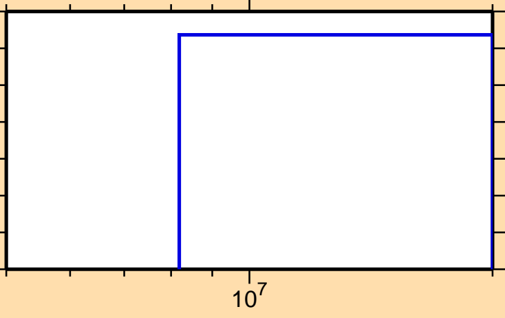
\sigma vs. E for ^{198}\text{Os}(n,t)
