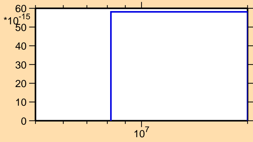
\sigma vs. E for ^{198}\text{Os}(n,2n\alpha)
