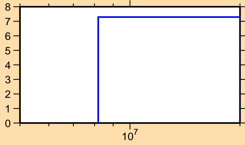
\Delta\sigma/\sigma vs. E for ^{198}\text{Os}(n,\text{el.})
