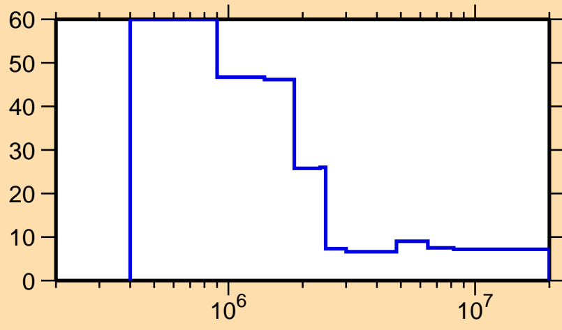
\Delta\sigma/\sigma vs. E for ^{198}\text{Os}(n,\text{nonel.})
