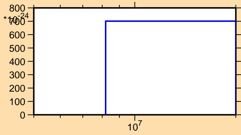
\sigma vs. E for ^{198}\text{Os} (mt 11)
