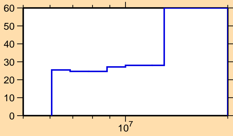
\Delta\sigma/\sigma vs. E for ^{200}\text{Os}(n,2n)
