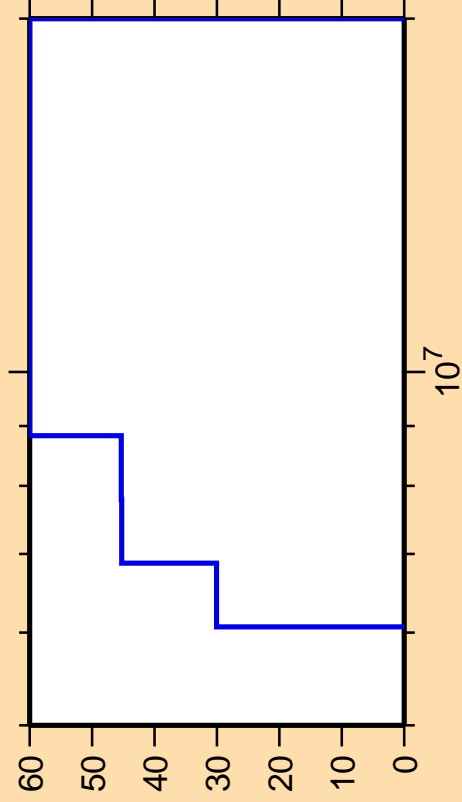
\Delta\sigma/\sigma vs. E for ^{200}\text{Os}(n,n\text{cont.})
