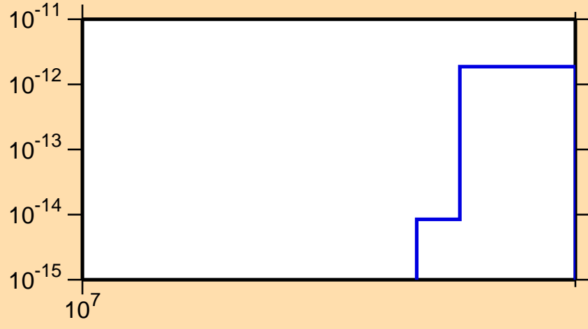
\sigma vs. E for ^{200}\text{Os}(n,2n\alpha)
