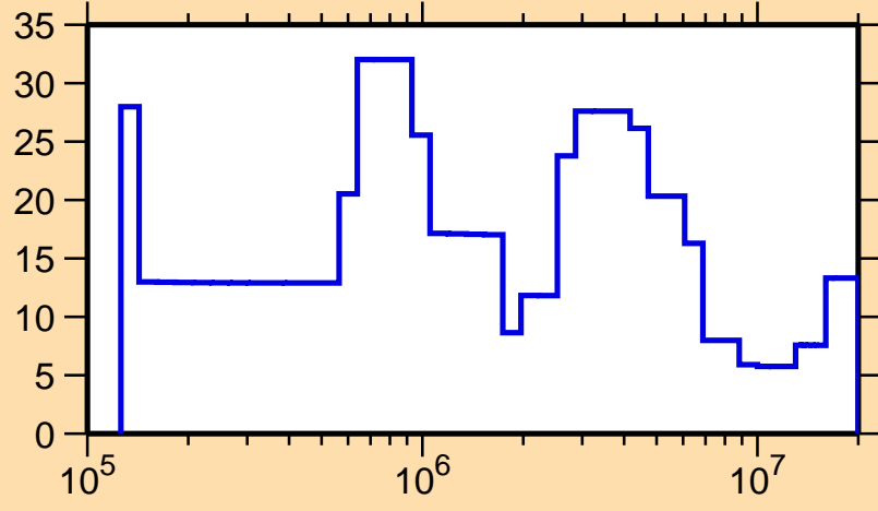
\Delta\sigma/\sigma vs. E for ^{200}\text{Os}(n,\text{tot.})
