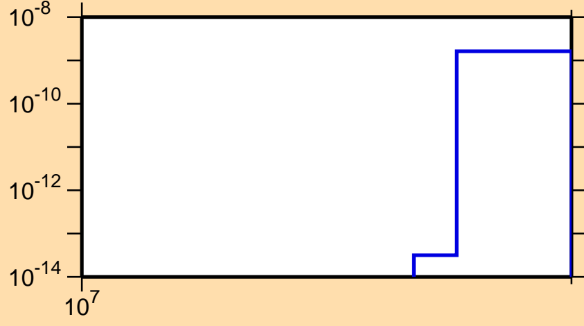
\sigma vs. E for ^{200}\text{Os}(n,nt)
