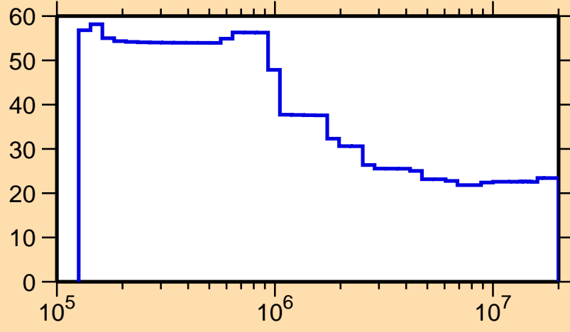
\Delta\sigma/\sigma vs. E for ^{200}\text{Os}(n,\text{nonel.})
