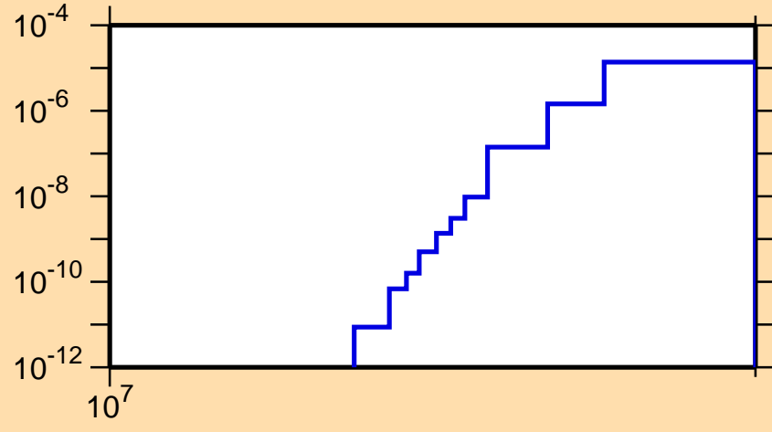
\sigma vs. E for ^{200}\text{Os}(n,t)
