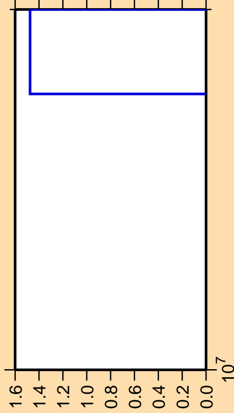
\Delta\sigma/\sigma vs. E for ^{200}\text{Os}(n,2np)
