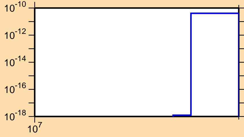
\sigma vs. E for ^{200}\text{Os}(n,\text{nd})
