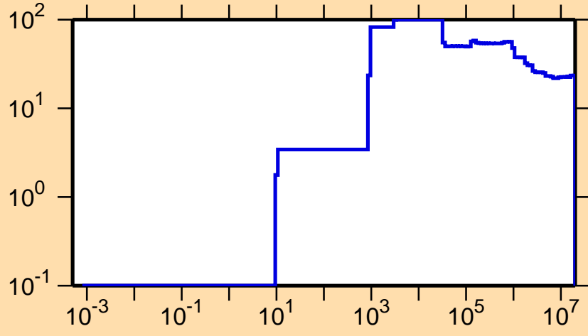
\Delta\sigma/\sigma vs. E for ^{200}\text{Os}(n,\text{nonel.})
