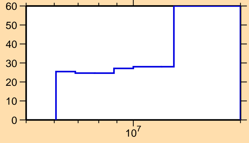
\Delta\sigma/\sigma vs. E for ^{200}\text{Os}(n,2n)
