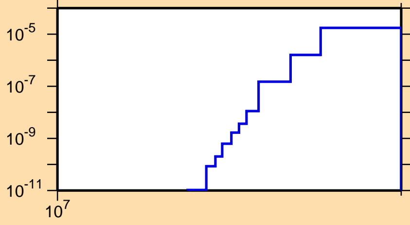
\sigma vs. E for ^{200}\text{Os}(n,d)
