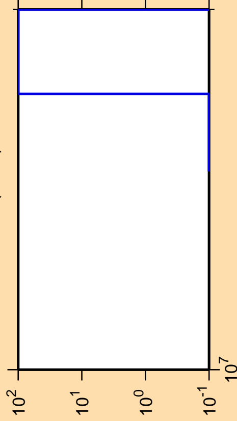
\Delta\sigma/\sigma vs. E for ^{200}\text{Os}(n,\text{nd})
