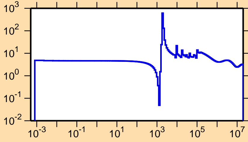
\sigma vs. E for ^{200}\text{Os}(n,\text{el.})
