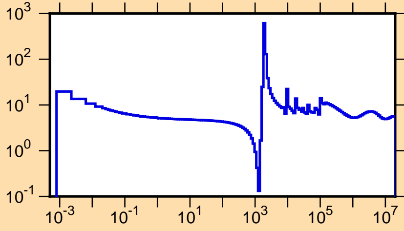
\sigma vs. E for ^{200}\text{Os}(n,\text{tot.})
