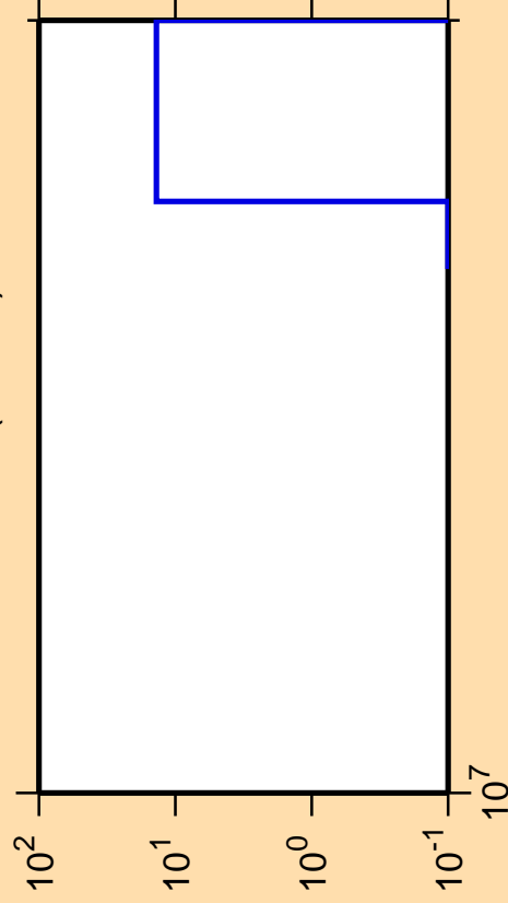
\Delta\sigma/\sigma vs. E for ^{200}\text{Os}(n,2n\alpha)
