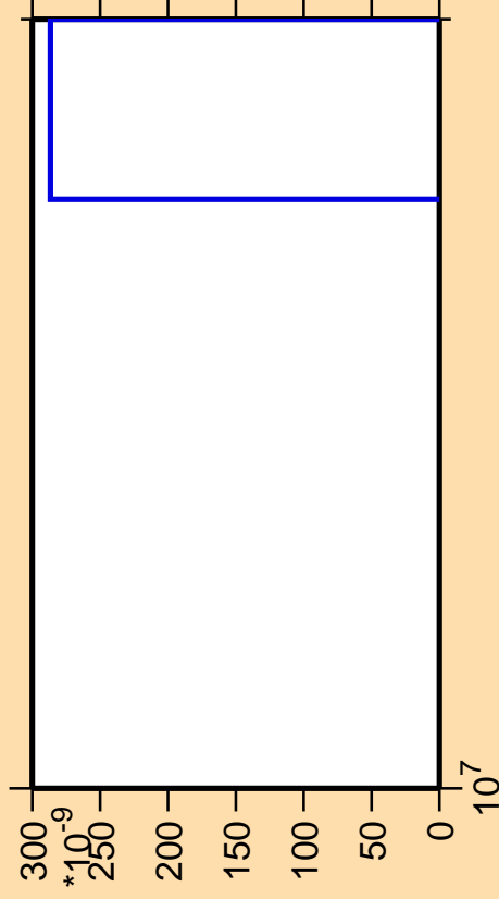
\Delta\sigma/\sigma vs. E for ^{200}\text{Os} (mt 11)
