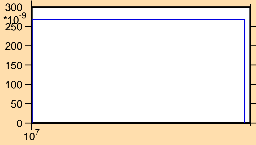
\sigma vs. E for ^{200}\text{Os}(n,d)
