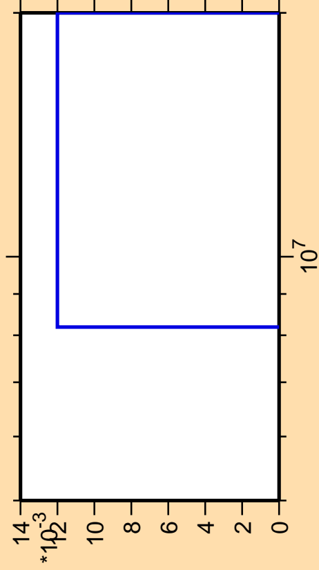
\Delta\sigma/\sigma vs. E for ^{200}\text{Os}(n,2np)
