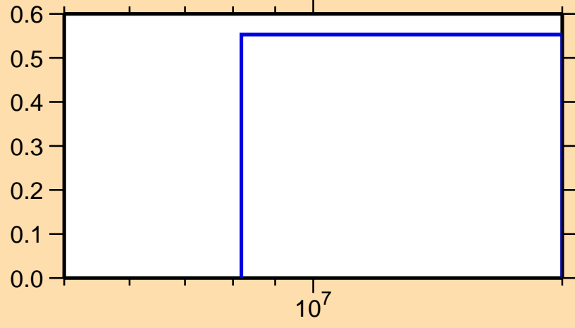
\sigma vs. E for ^{200}\text{Os}(n,3n)
