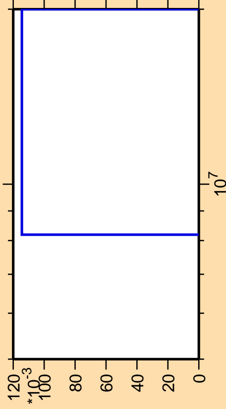
\Delta\sigma/\sigma vs. E for ^{200}\text{Os}(n,2n\alpha)
