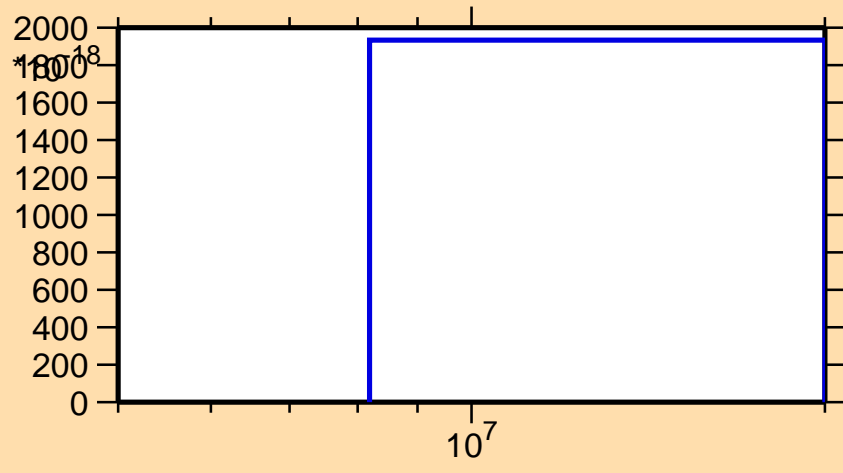
\sigma vs. E for ^{200}\text{Os}(n,2np)
