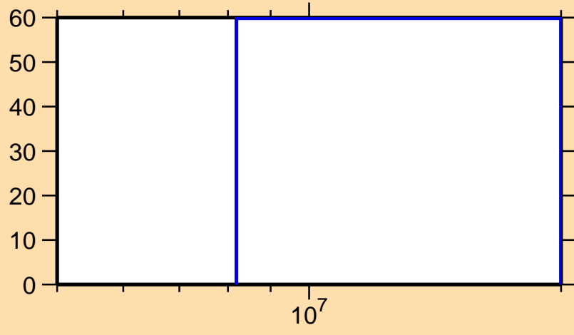
\Delta\sigma/\sigma vs. E for ^{200}\text{Os}(n,ncont.)
