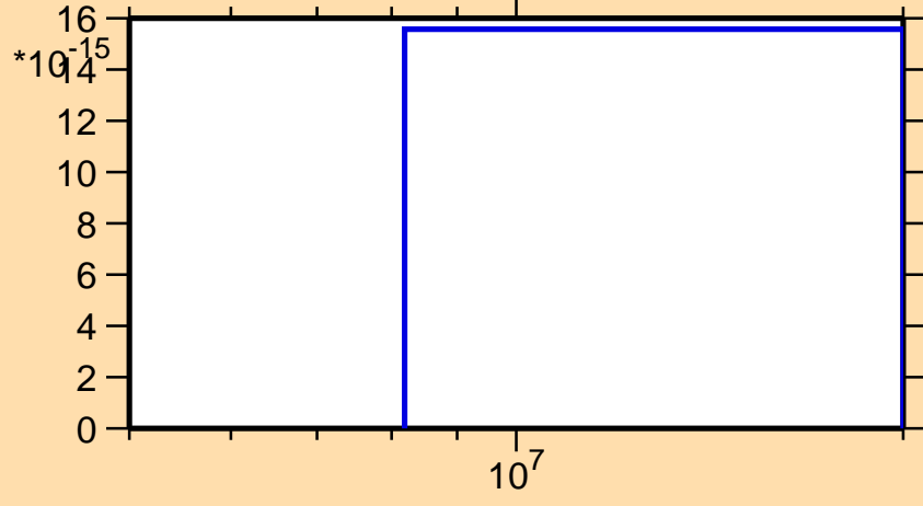
\sigma vs. E for ^{200}\text{Os}(n,2n\alpha)
