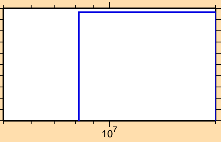
\sigma vs. E for ^{200}\text{Os}(n,p)
