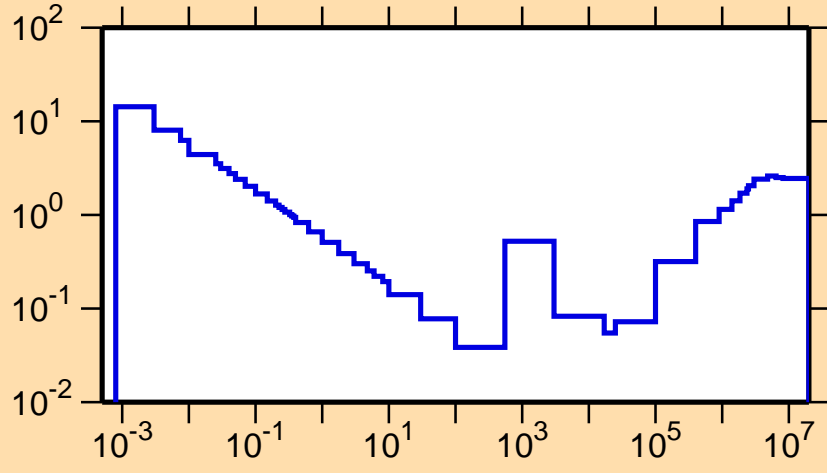
\sigma vs. E for ^{200}\text{Os}(n,\text{nonel.})
