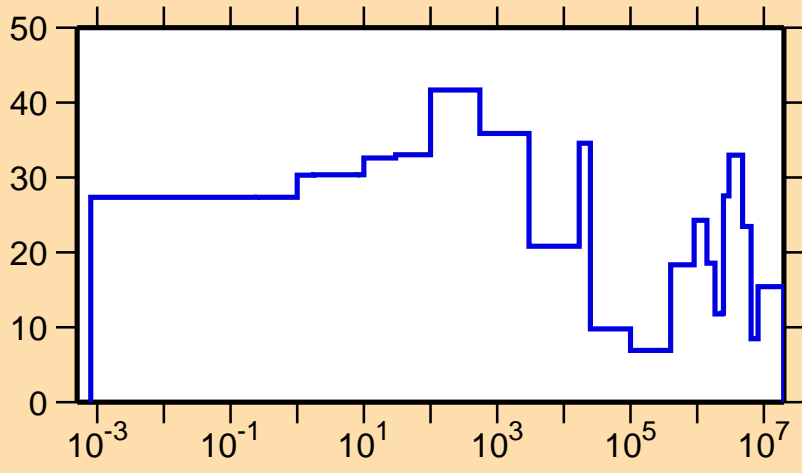
\Delta\sigma/\sigma vs. E for ^{200}\text{Os}(n,\text{el.})
