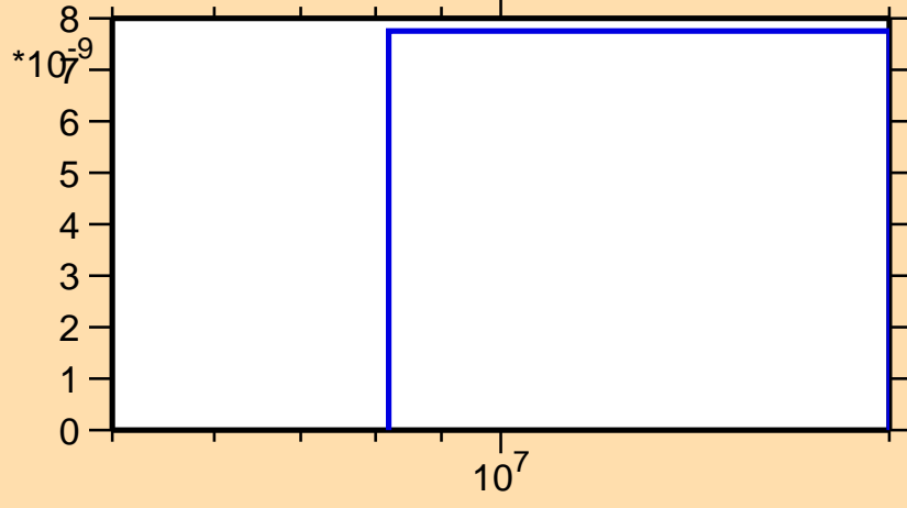
\sigma vs. E for ^{200}\text{Os}(n,n\alpha)
