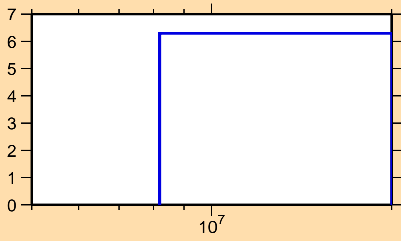
\Delta\sigma/\sigma vs. E for ^{200}\text{Os}(n,\text{tot.})
