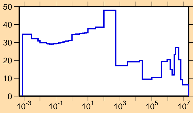
\Delta\sigma/\sigma vs. E for ^{200}\text{Os}(n,\text{tot.})
