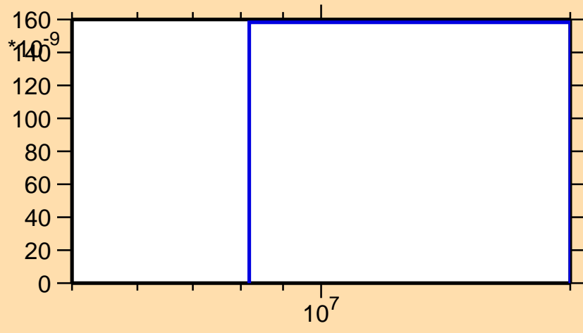
\sigma vs. E for ^{200}\text{Os}(n,np)
