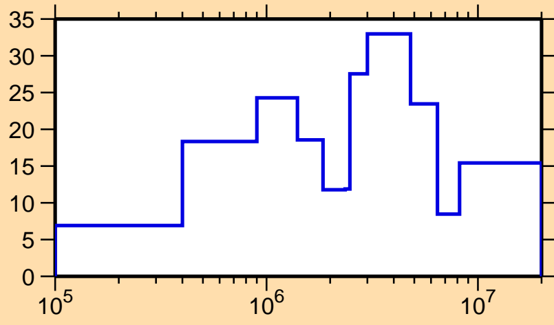
\Delta\sigma/\sigma vs. E for ^{200}\text{Os}(n, el.)
