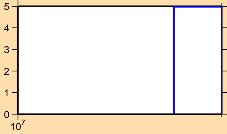
\Delta\sigma/\sigma vs. E for ^{29}\text{P}(n,\text{tot.})
