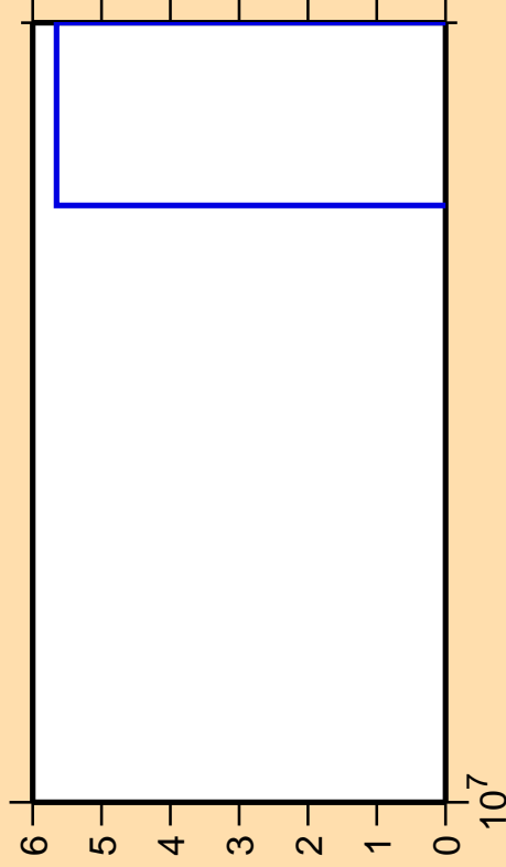
\Delta\sigma/\sigma vs. E for ^{29}\text{P}(n,\text{pt})
