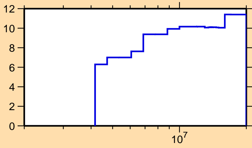
\Delta\sigma/\sigma vs. E for ^{29}\text{P}(n,n\text{onel.})
