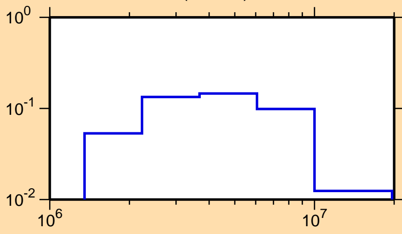
\sigma vs. E for ^{29}\text{P}(n,\text{inel.})
