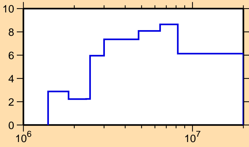
\Delta\sigma/\sigma vs. E for ^{29}\text{P}(n,\text{tot.})
