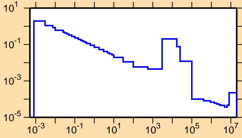
\sigma vs. E for ^{29}\text{P}(n,\gamma)
