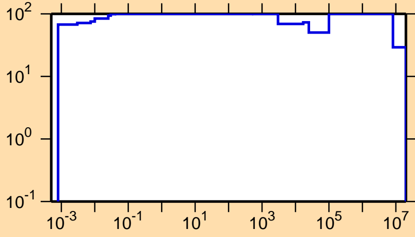
\Delta\sigma/\sigma vs. E for ^{29}\text{P}(n,\gamma)
