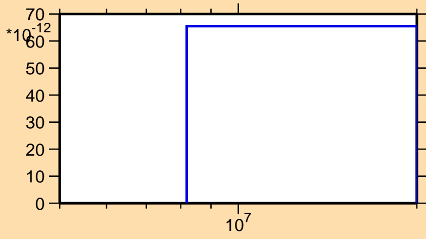
\sigma vs. E for ^{29}\text{P}(n,\text{nd})
