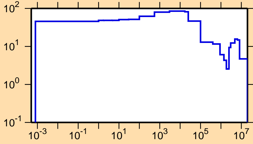
\Delta\sigma/\sigma vs. E for ^{29}\text{P}(n,el.)
