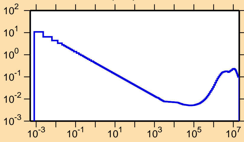
\sigma vs. E for ^{30}\text{P}(n,\alpha)
