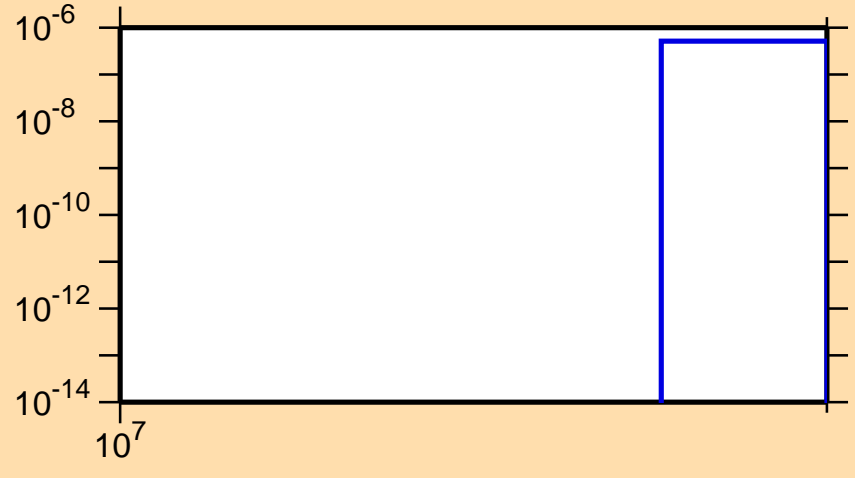
\sigma vs. E for ^{30}\text{P}(n,pd)
