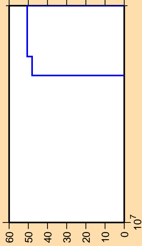
\Delta\sigma/\sigma vs. E for ^{30}\text{P}(n,pd)
