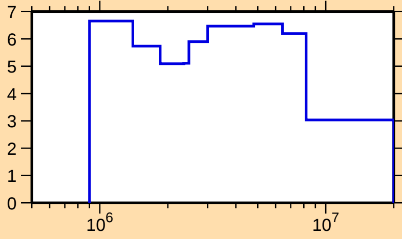
\Delta\sigma/\sigma vs. E for ^{31}\text{P}(\text{n,tot.})
