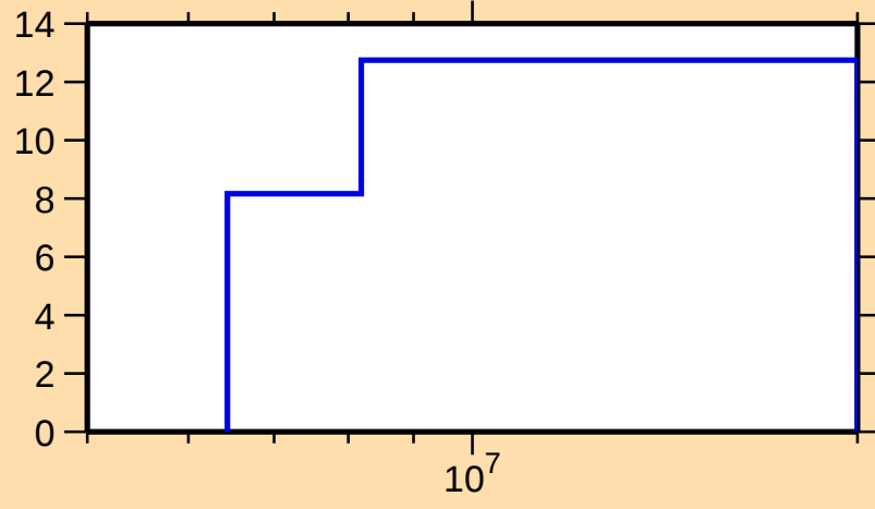
\Delta\sigma/\sigma vs. E for ^{31}\text{P}(\text{n},\text{inel.})
