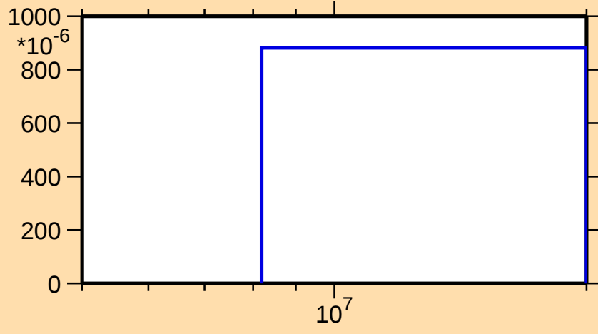
\sigma vs. E for ^{31}\text{P}(n,t)
