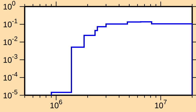
\sigma vs. E for ^{31}\text{P}(n,p)
