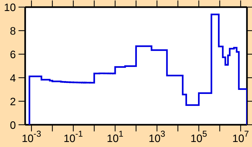
\Delta\sigma/\sigma vs. E for ^{31}\text{P}(\text{n,tot.})
