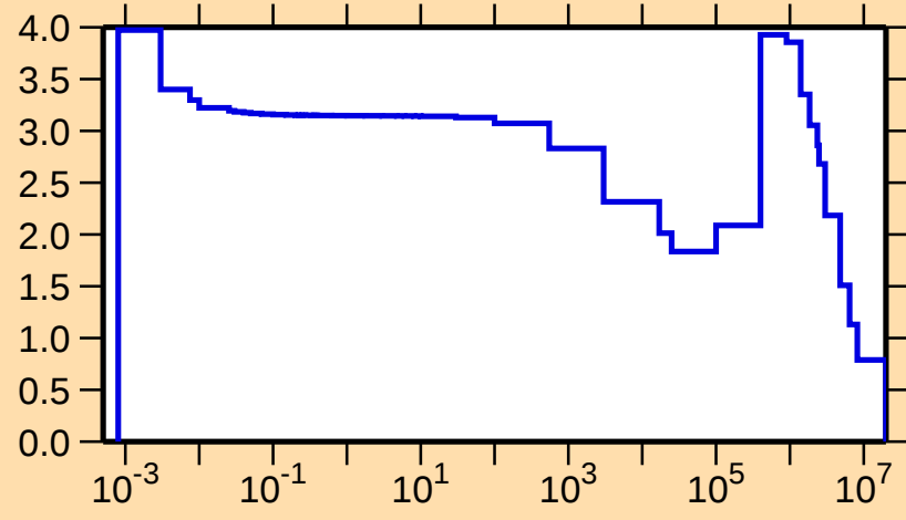
\sigma vs. E for ^{31}\text{P}(\text{n,el.})
