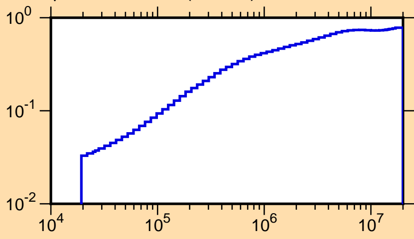
\mu vs. E for ^{32}\text{P} (mt251)
