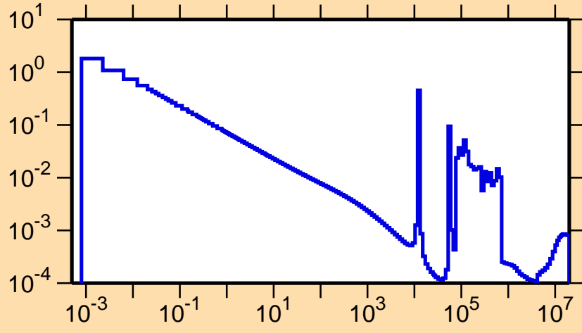
\sigma vs. E for ^{32}\text{P}(n,\gamma)
