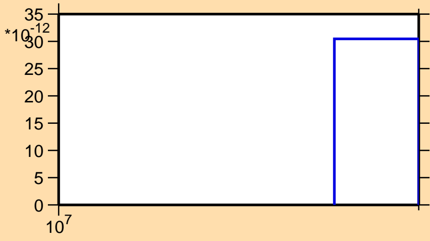
\sigma vs. E for ^{32}\text{P}(n,2n\alpha)
