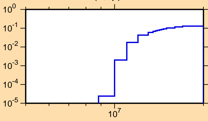
\sigma vs. E for ^{32}\text{P}(n,np)
