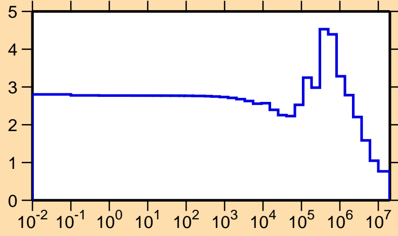
\sigma vs. E for ^{32}\text{P}(n,\text{el.})
