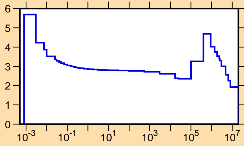
\sigma vs. E for ^{32}\text{P}(n,\text{tot.})
