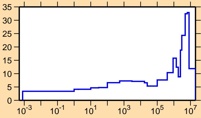
\Delta\sigma/\sigma vs. E for ^{32}\text{P}(n,el.)
