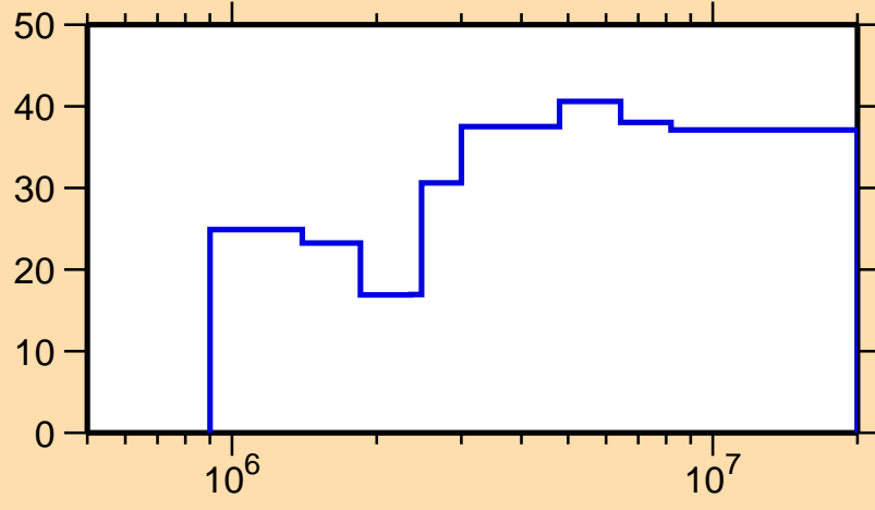
\Delta\sigma/\sigma vs. E for ^{32}\text{P}(n,p)
