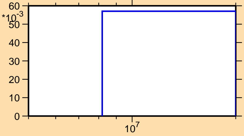
\sigma vs. E for ^{32}\text{P}(n,np)
