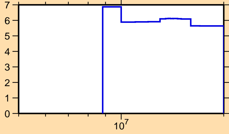
\Delta\sigma/\sigma vs. E for ^{35}\text{P}(n,el.)
