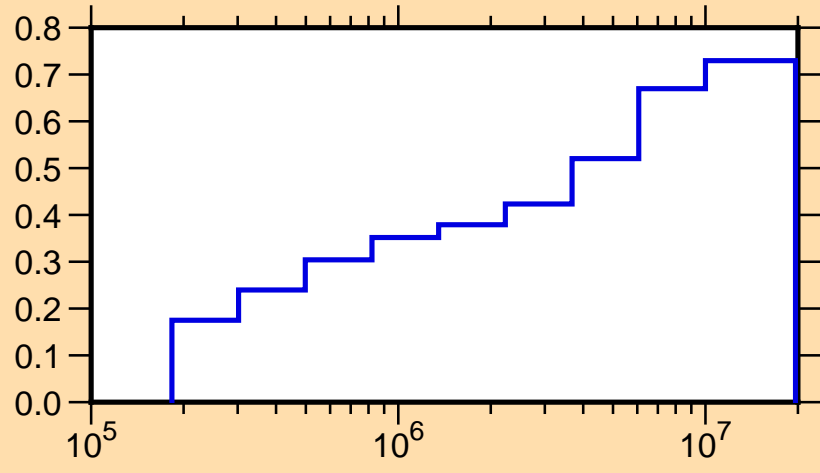
\mu vs. E for ^{35}\text{P}(\text{mt251})
