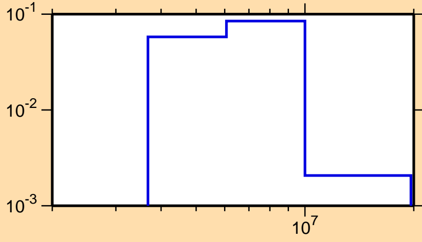
\sigma vs. E for ^{35}\text{P}(n,n_3)
