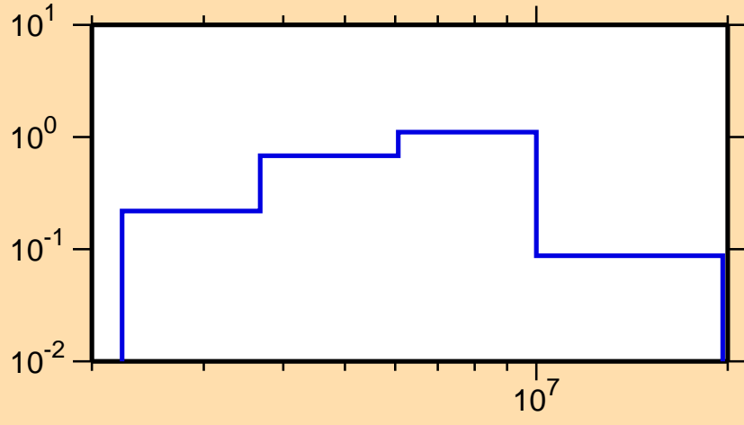
\sigma vs. E for ^{35}\text{P}(n,\text{inel.})
