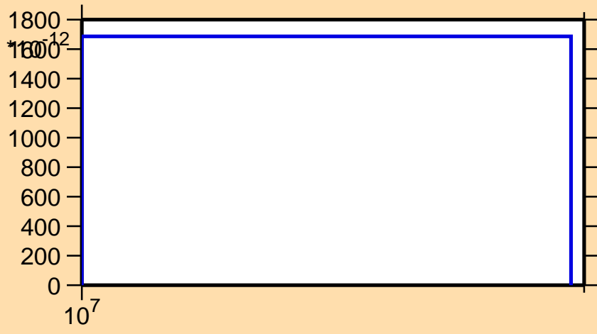
\sigma vs. E for ^{35}\text{P}(n,\text{nd})
