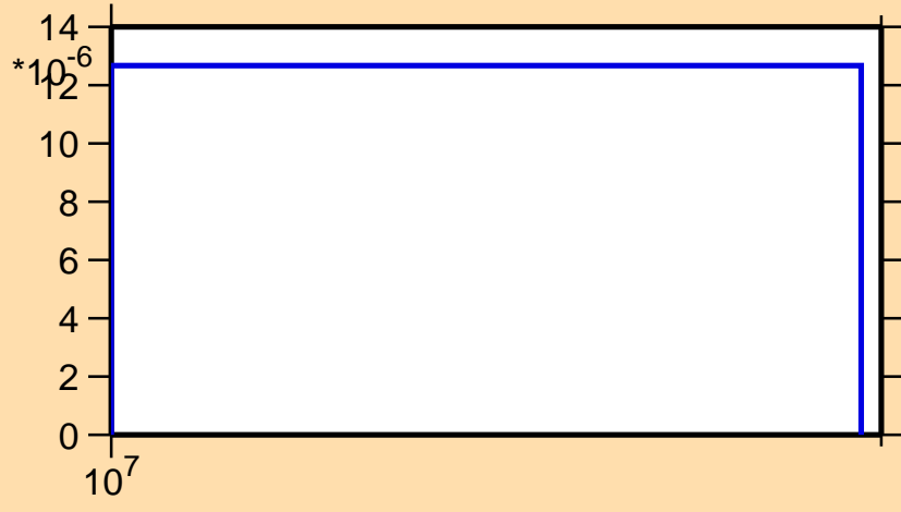
\sigma vs. E for ^{35}\text{P}(n,n\alpha)
