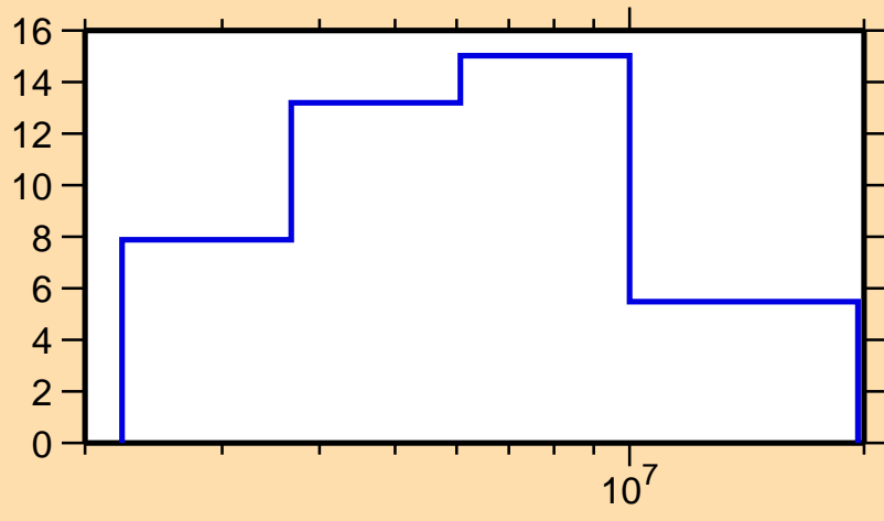
\Delta\sigma/\sigma vs. E for ^{35}\text{P}(n,\text{el.})
