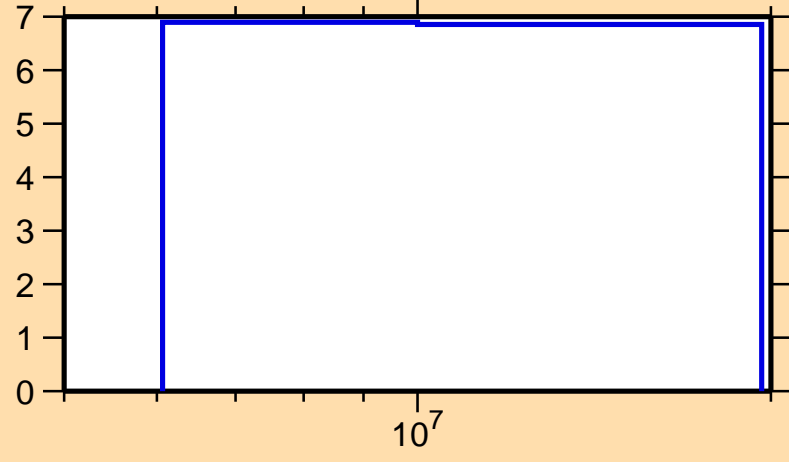
\Delta\sigma/\sigma vs. E for ^{35}\text{P}(n,n\text{onel.})
