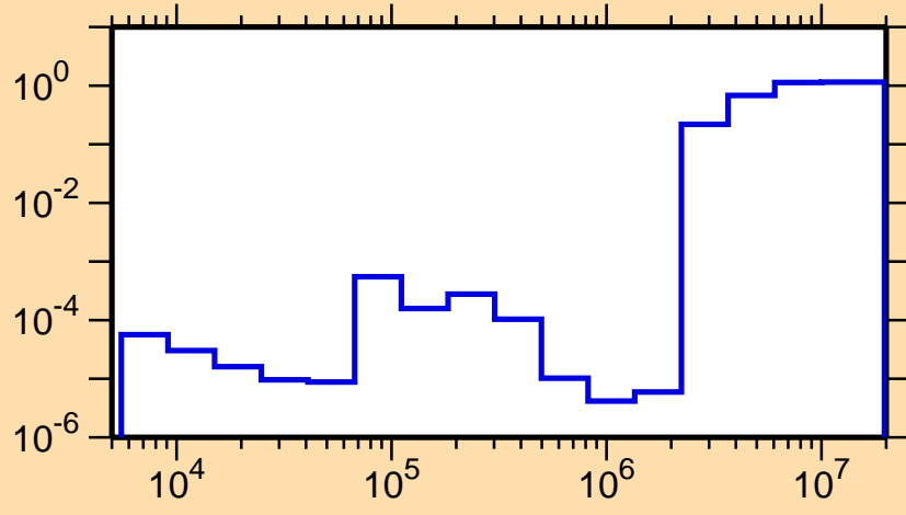
\sigma vs. E for ^{35}\text{P}(n,\text{nonel.})
