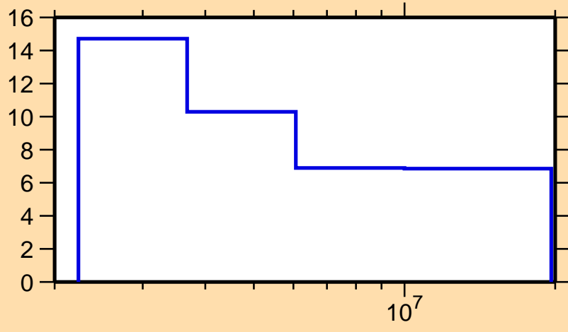
\Delta\sigma/\sigma vs. E for ^{35}\text{P}(n,\text{nonel.})
