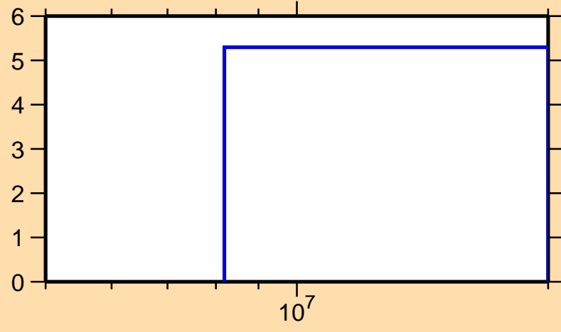
\Delta\sigma/\sigma vs. E for ^{35}\text{P}(n,\text{tot.})
