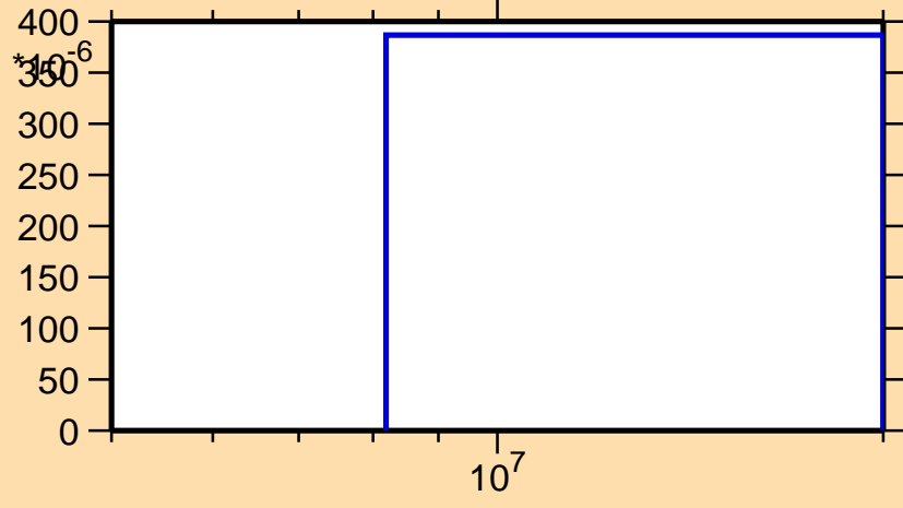
\sigma vs. E for ^{35}\text{P}(n,\alpha)
