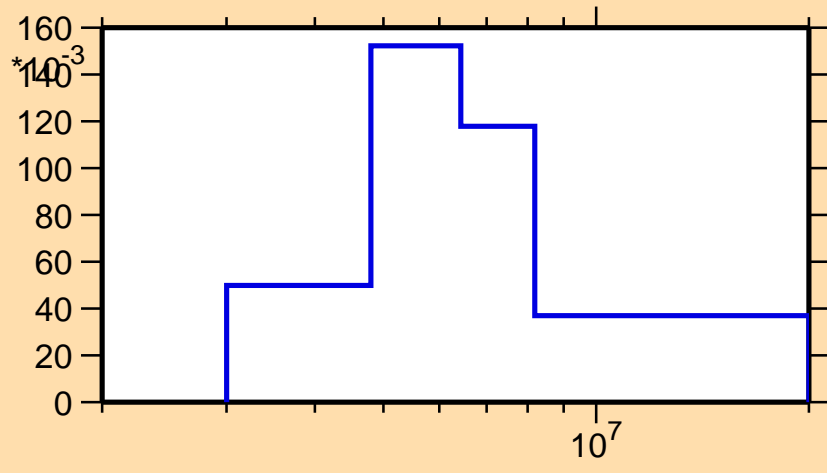
\sigma vs. E for ^{35}\text{P}(n,n_2)
