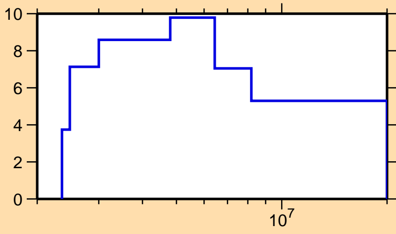
\Delta\sigma/\sigma vs. E for ^{35}\text{P}(n,\text{tot.})
