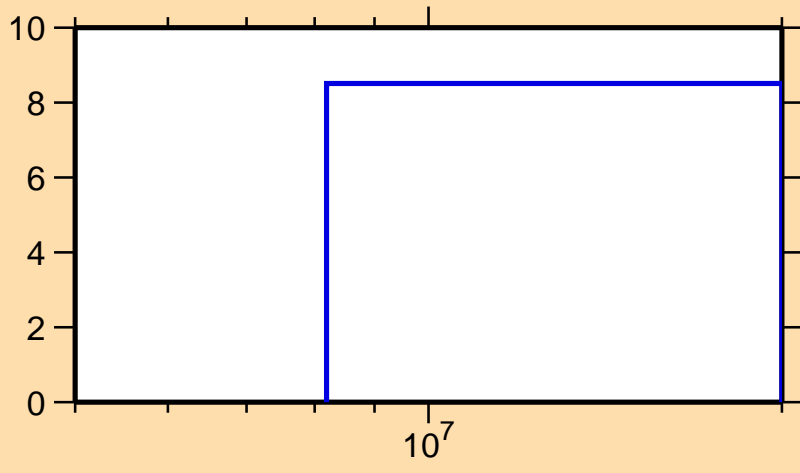
\Delta\sigma/\sigma vs. E for ^{35}\text{P}(n,2n)
