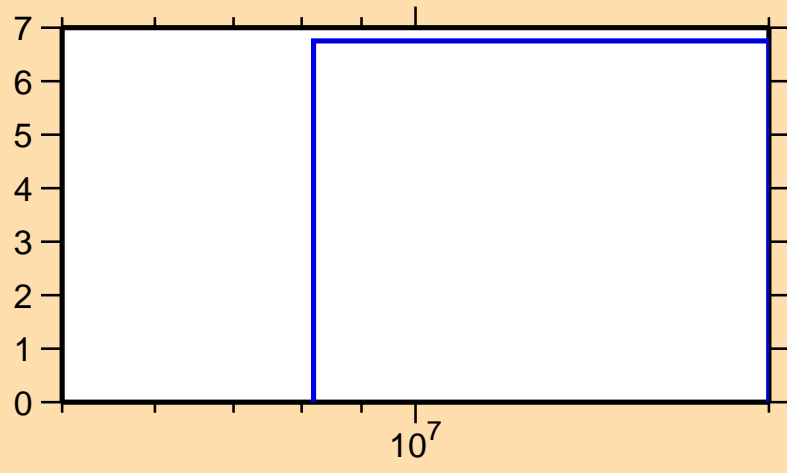
\Delta\sigma/\sigma vs. E for ^{35}\text{P}(n,\text{nonel.})
