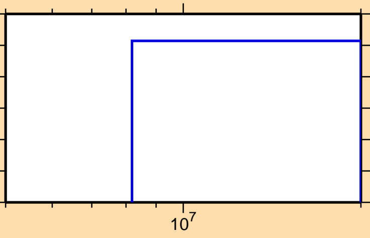
\sigma vs. E for ^{35}\text{P}(n,n\alpha)
