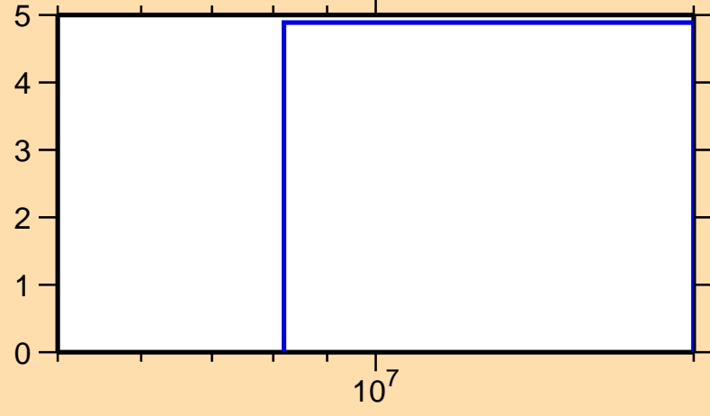
\Delta\sigma/\sigma vs. E for ^{35}\text{P}(n,\text{el.})
