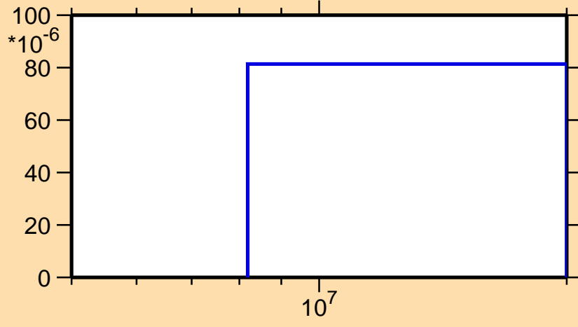
\sigma vs. E for ^{35}\text{P}(n,t)
