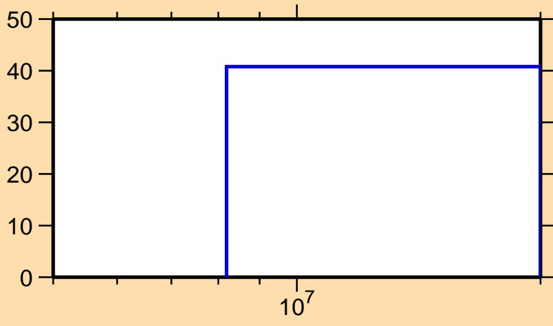
\Delta\sigma/\sigma vs. E for ^{35}\text{P}(n,n_1)
