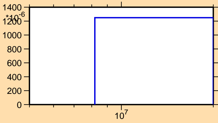
\sigma vs. E for ^{35}\text{P}(n,p)
