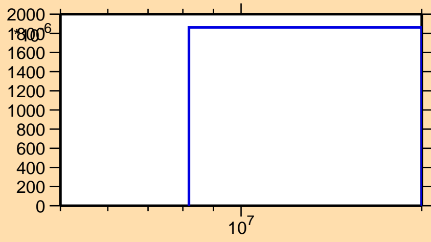
\sigma vs. E for ^{35}\text{P}(n,3n)
