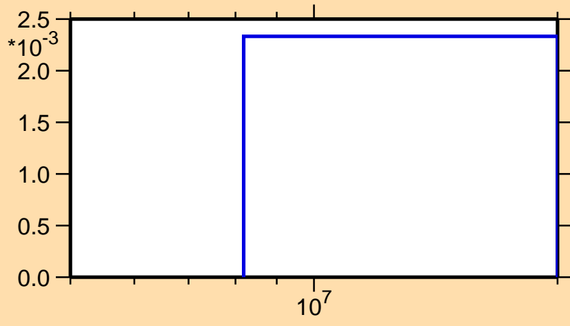
\sigma vs. E for ^{35}\text{P}(n,n\text{cont.})
