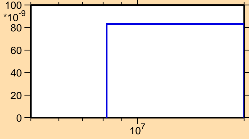
\sigma vs. E for ^{35}\text{P}(n,nt)
