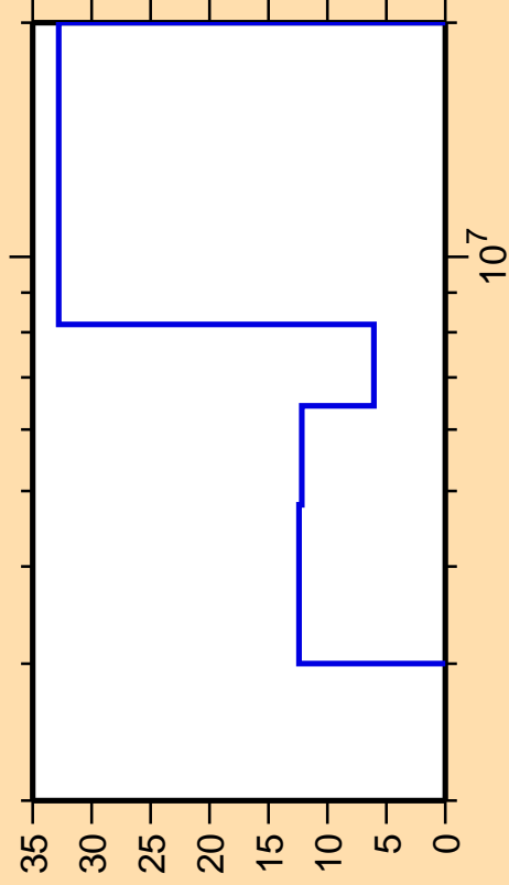
\Delta\sigma/\sigma vs. E for ^{35}\text{P}(n,n_4)
