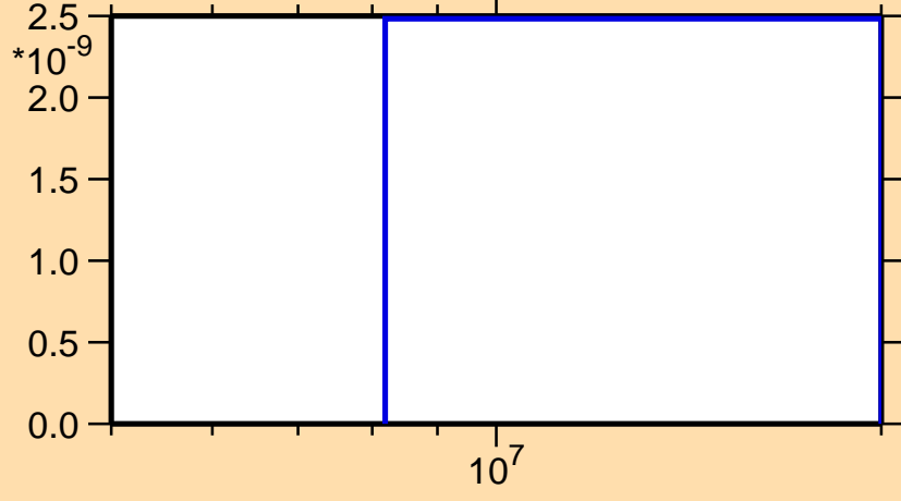
\sigma vs. E for ^{35}\text{P}(n,\text{nd})
