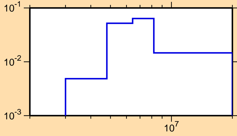
\sigma vs. E for ^{35}\text{P}(n,n_4)
