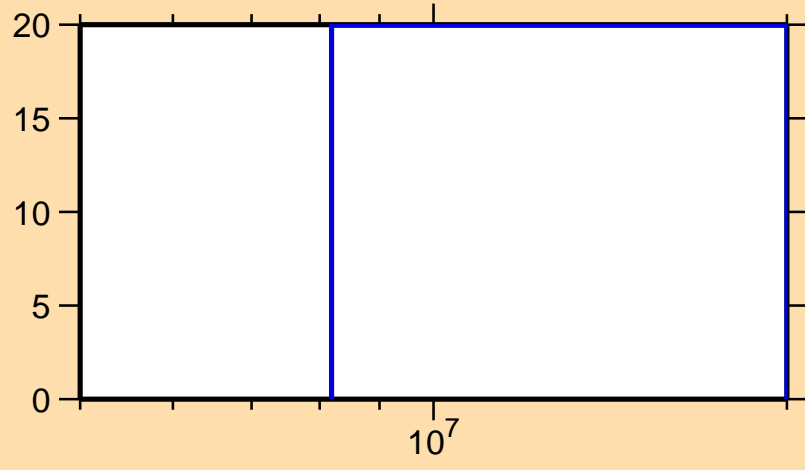
\Delta\sigma/\sigma vs. E for ^{35}\text{P}(n,\text{inel.})
