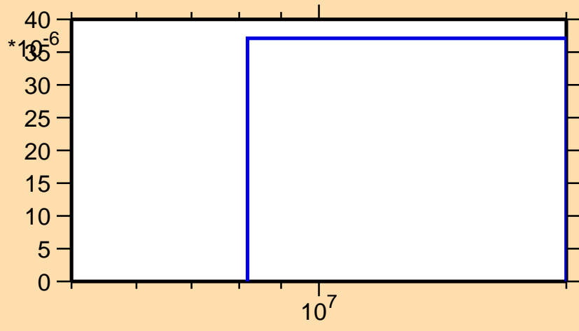
\sigma vs. E for ^{35}\text{P}(n,np)
