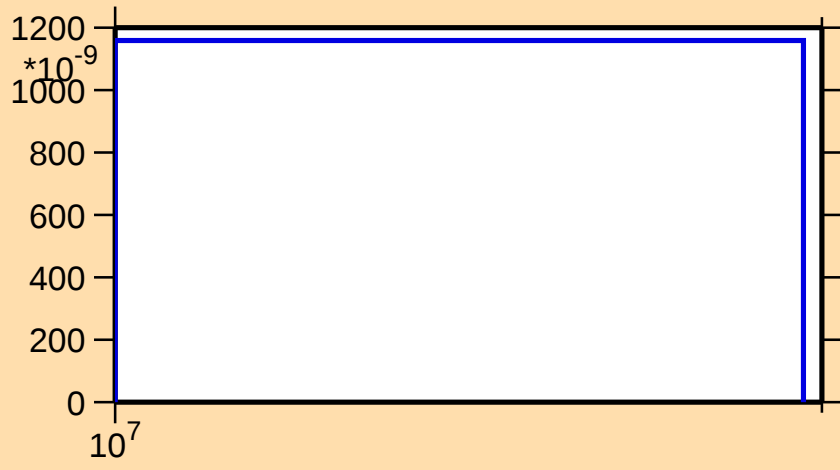
\sigma vs. E for ^{37}\text{P}(\text{n,np})
