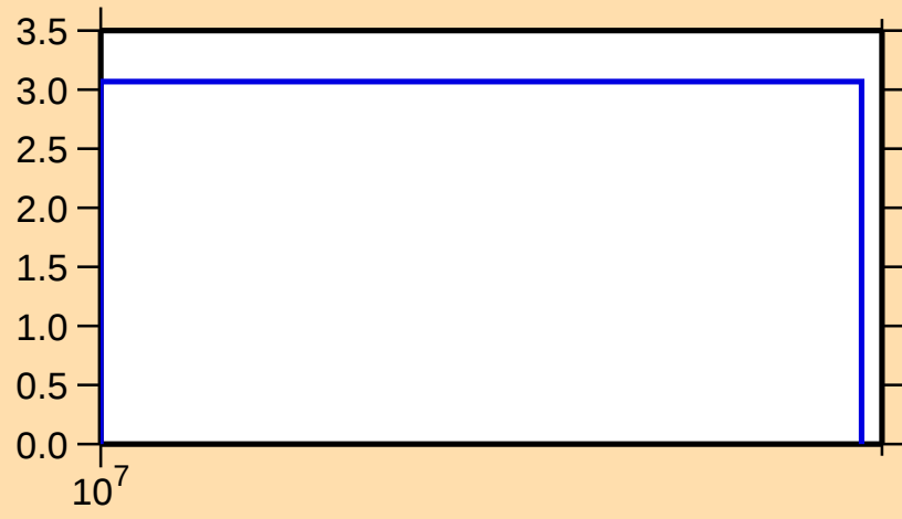
\Delta\sigma/\sigma vs. E for ^{37}\text{P}(\text{n,tot.})
