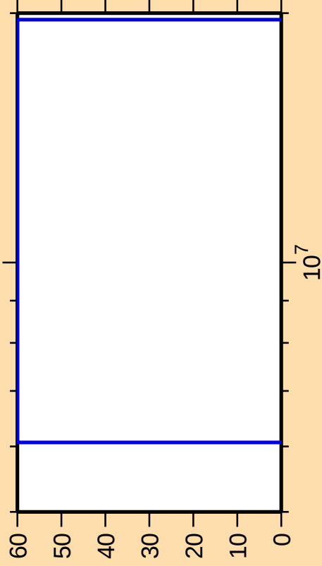
\Delta\sigma/\sigma vs. E for ^{37}\text{P}(n,\gamma)
