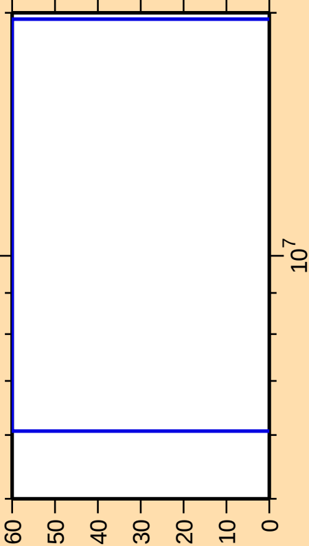
\Delta\sigma/\sigma vs. E for ^{37}\text{P}(n,\gamma)
