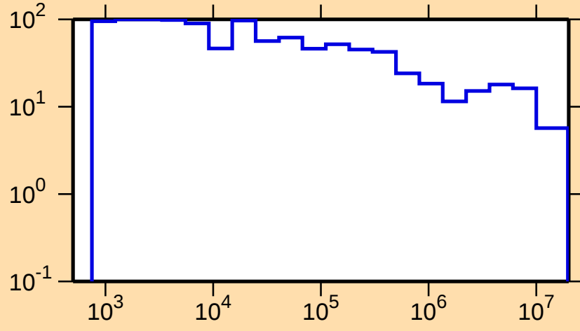
\Delta\sigma/\sigma vs. E for ^{37}\text{P}(\text{n,el.})
