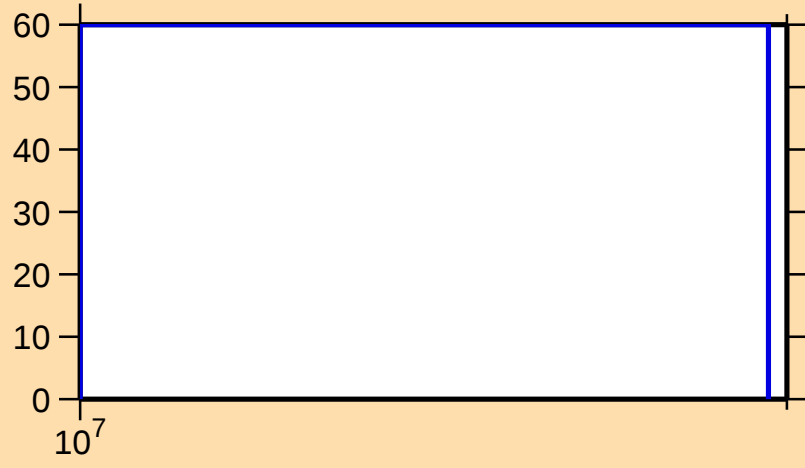
\Delta\sigma/\sigma vs. E for ^{37}\text{P}(\text{n,ncont.})
