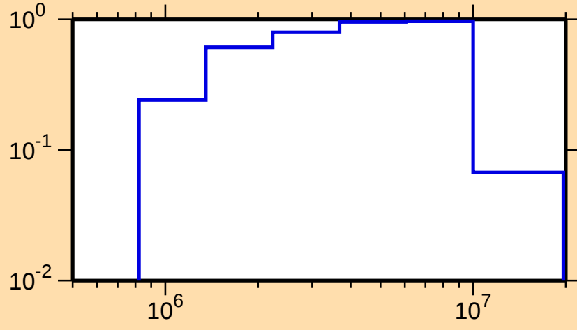
\sigma vs. E for ^{37}\text{P}(\text{n,inel.})
