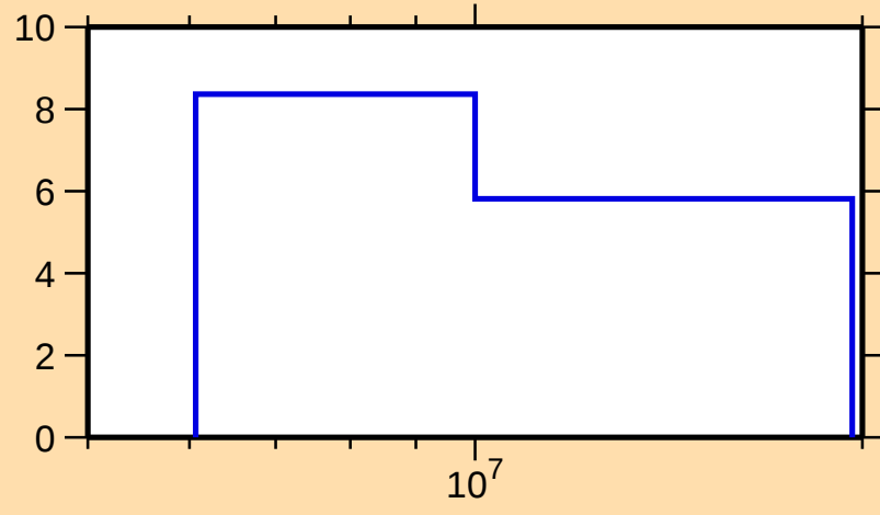
\Delta\sigma/\sigma vs. E for ^{37}\text{P}(\text{n},\text{nonel.})
