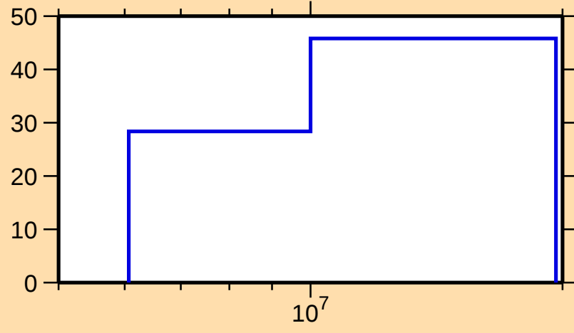
\Delta\sigma/\sigma vs. E for ^{37}\text{P}(\text{n},\text{inel.})
