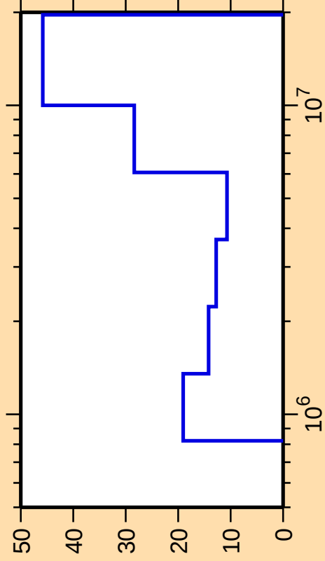
\Delta\sigma/\sigma vs. E for ^{37}\text{P}(\text{n,inel.})
