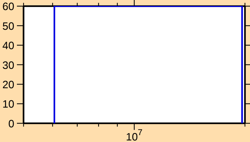
\Delta\sigma/\sigma vs. E for ^{37}\text{P}(n,\text{ncont.})
