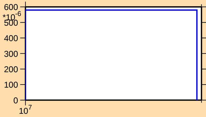
\sigma vs. E for ^{37}\text{P}(\text{n,d})
