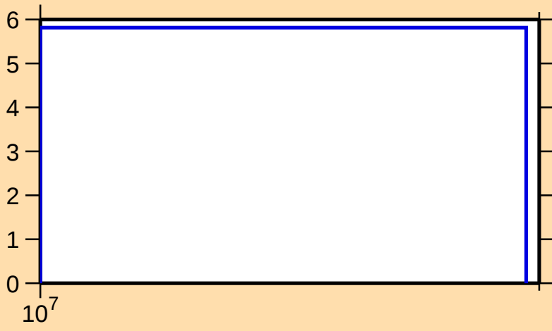
\Delta\sigma/\sigma vs. E for ^{37}\text{P}(\text{n,nonel.})
