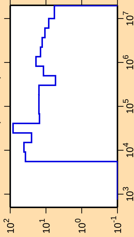
\Delta\sigma/\sigma vs. E for ^{37}\text{P}(\text{n,nonel.})
