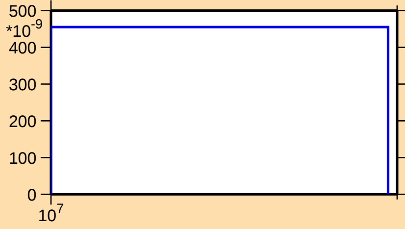
\sigma vs. E for ^{37}\text{P}(\text{n},\text{nt})
