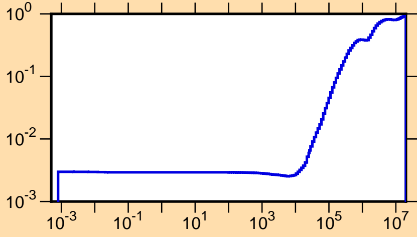
\mu vs. E for ^{225}\text{Pa}(\text{mt251})
