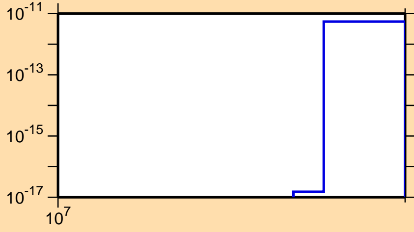
\sigma vs. E for ^{225}\text{Pa} (mt 11)
