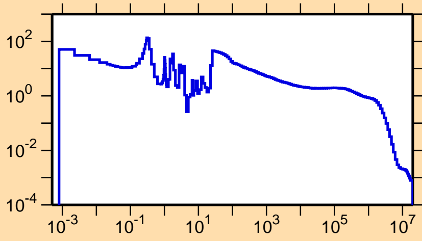
\sigma vs. E for ^{225}\text{Pa}(n,\gamma)
