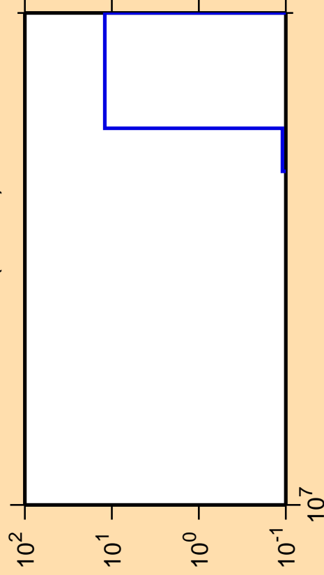
\Delta\sigma/\sigma vs. E for ^{225}\text{Pa} (mt 34)
