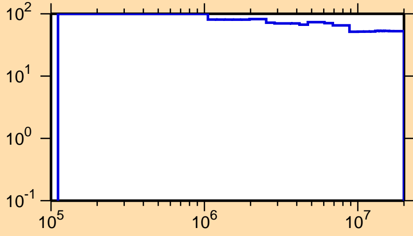
\Delta\sigma/\sigma vs. E for ^{225}\text{Pa}(n,n\text{cont.})
