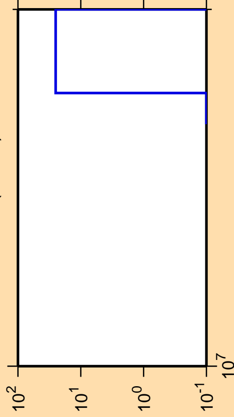
\Delta\sigma/\sigma vs. E for ^{225}\text{Pa} (mt 11)
