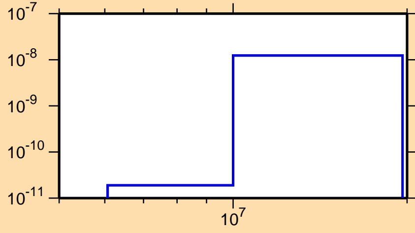
\sigma vs. E for ^{225}\text{Pa}(n,p\alpha)
