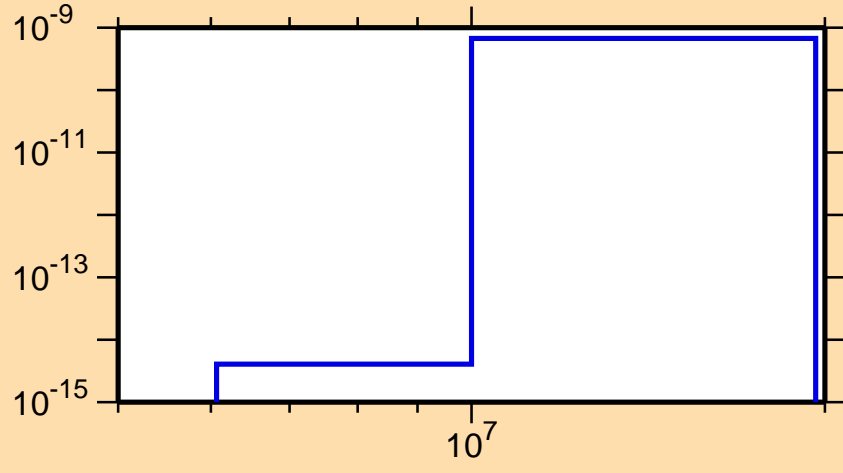
\sigma vs. E for ^{225}\text{Pa}(\text{mt117})
