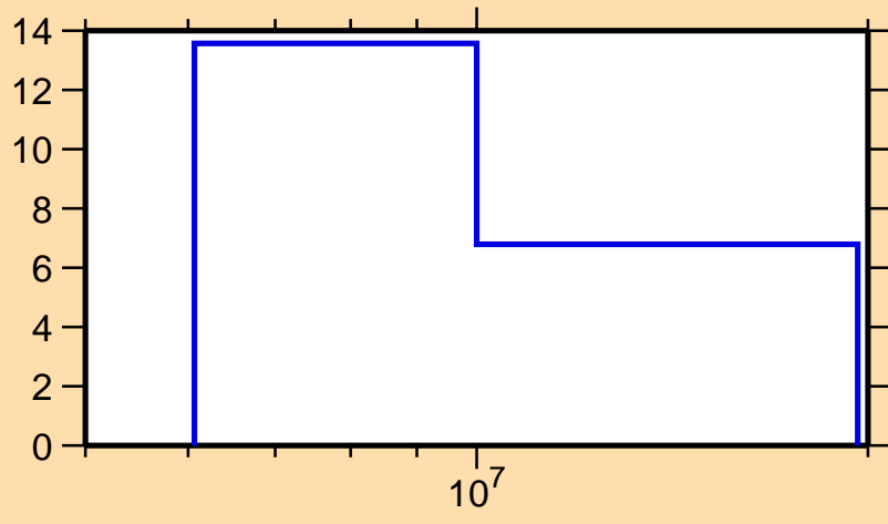
\Delta\sigma/\sigma vs. E for ^{225}\text{Pa}(n,\text{tot.})
