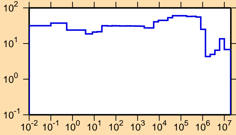
\Delta\sigma/\sigma vs. E for ^{225}\text{Pa}(n,tot.)
