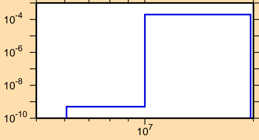
\sigma vs. E for ^{225}\text{Pa}(n,t)
