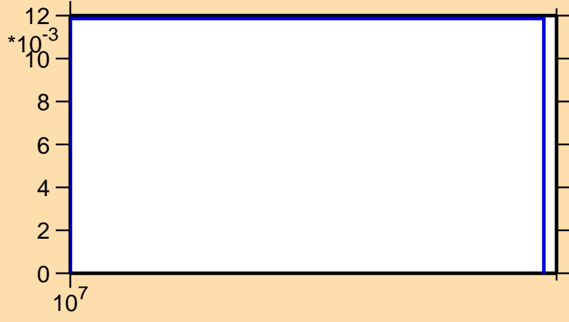
\sigma vs. E for ^{225}\text{Pa}(n,3n)
