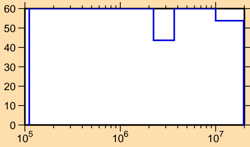
\Delta\sigma/\sigma vs. E for ^{225}\text{Pa}(n,n_1)
