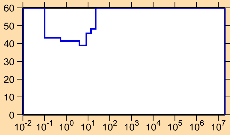
\Delta\sigma/\sigma vs. E for ^{225}\text{Pa}(n,\gamma)
