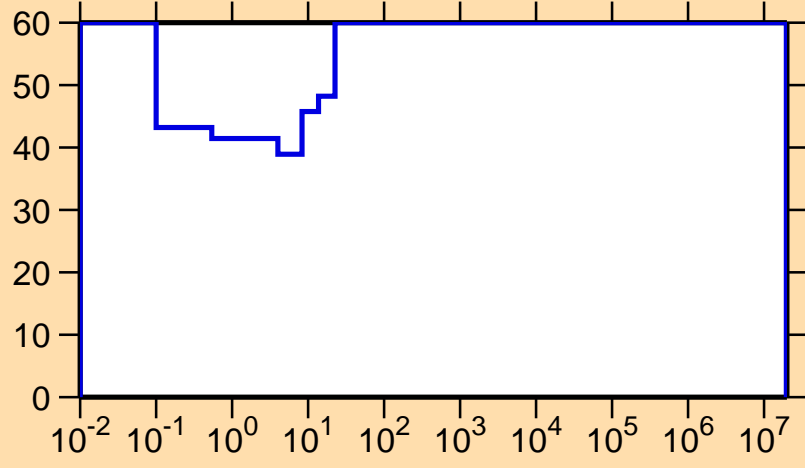
\Delta\sigma/\sigma vs. E for ^{225}\text{Pa}(n,\gamma)
