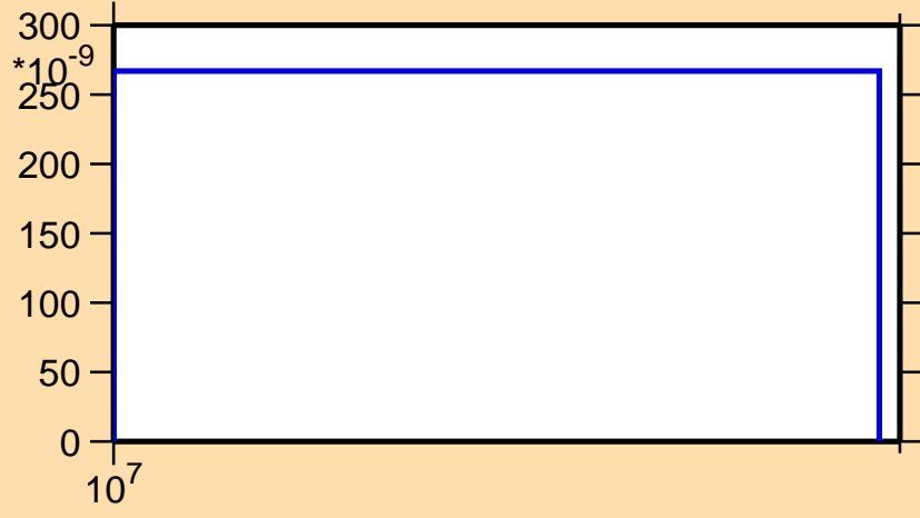
\sigma vs. E for ^{225}\text{Pa}(n,2np)
