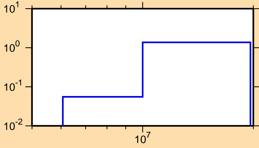
\sigma vs. E for ^{225}\text{Pa}(n,2n)
