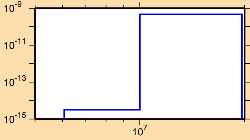
\sigma vs. E for ^{225}\text{Pa} (mt 45)
