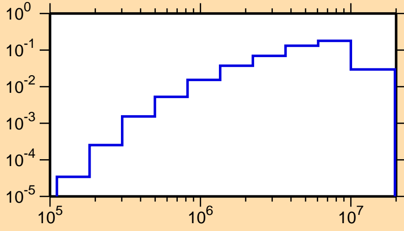
\sigma vs. E for ^{225}\text{Pa}(n,n\alpha)
