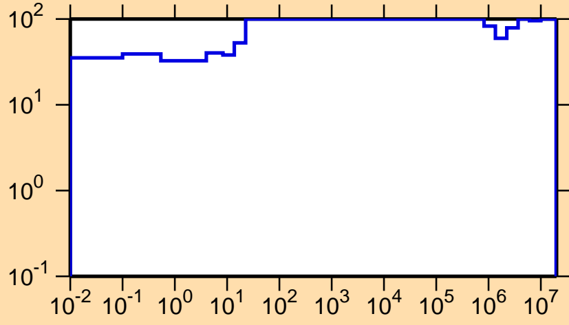
\Delta\sigma/\sigma vs. E for ^{225}\text{Pa}(n,f)
