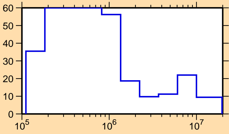
\Delta\sigma/\sigma vs. E for ^{225}\text{Pa}(n,\text{el.})
