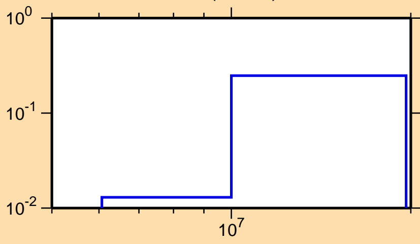
\sigma vs. E for ^{225}\text{Pa}(n,2n\alpha)
