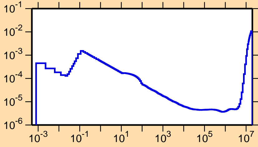
\sigma vs. E for ^{226}\text{Pa}(n,\alpha)
