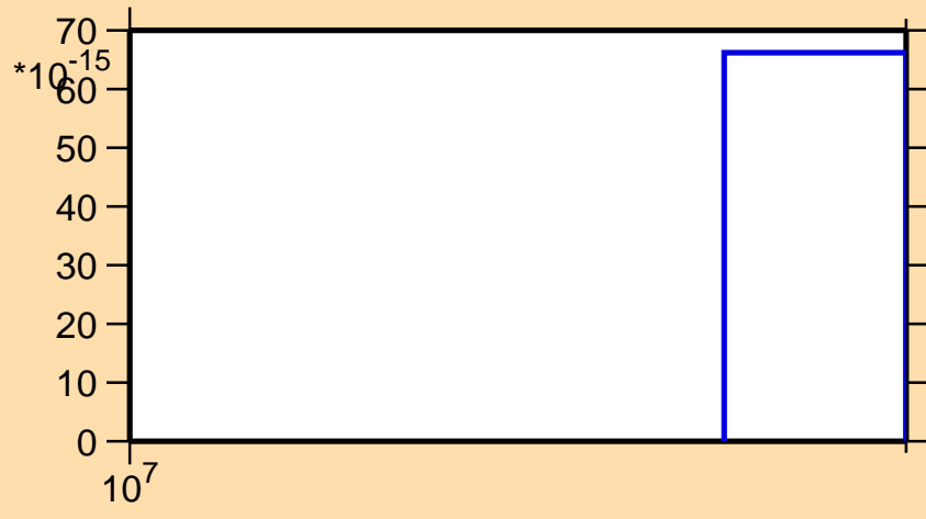
\sigma vs. E for ^{226}\text{Pa} (mt 42)
