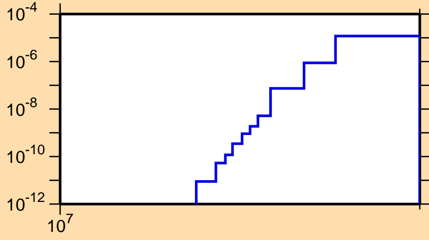
\sigma vs. E for ^{226}\text{Pa}(n,nt)
