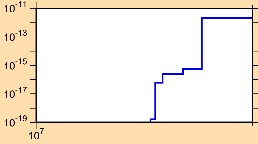
\sigma vs. E for ^{226}\text{Pa} (mt 11)
