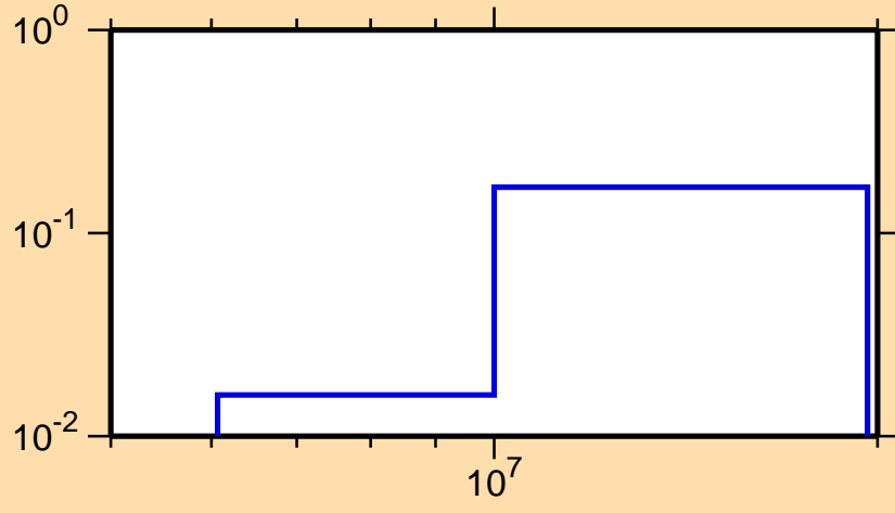
\sigma vs. E for ^{226}\text{Pa}(n,2n\alpha)
