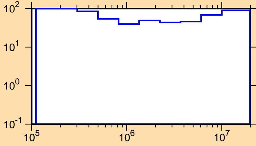
\Delta\sigma/\sigma vs. E for ^{226}\text{Pa}(n,n\text{cont.})
