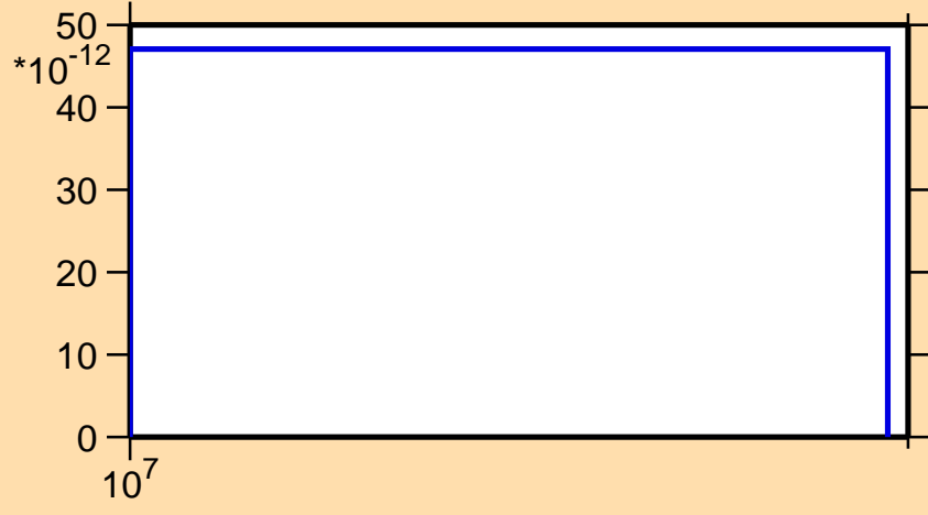
\sigma vs. E for ^{226}\text{Pa} (mt 45)
