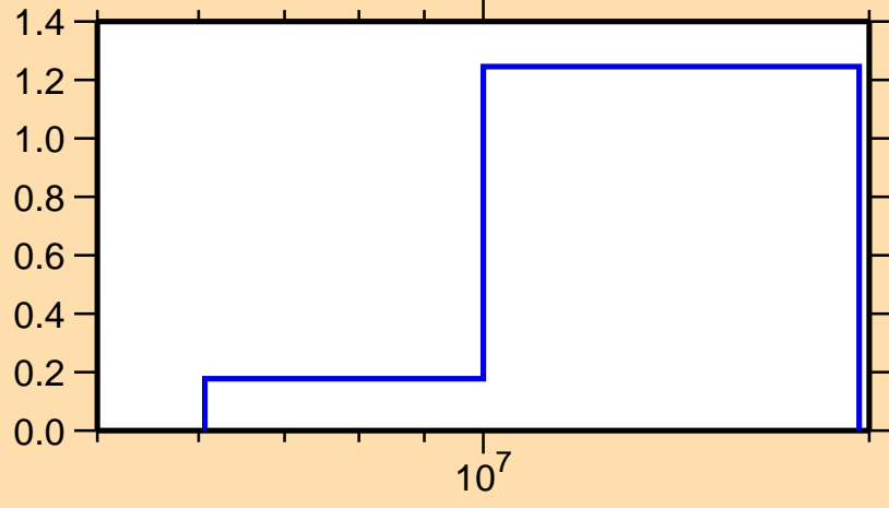
\sigma vs. E for ^{226}\text{Pa}(n,2n)
