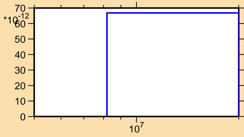
\sigma vs. E for ^{226}\text{Pa}(\text{mt117})
