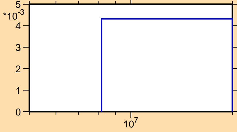
\sigma vs. E for ^{226}\text{Pa}(n,3n\alpha)
