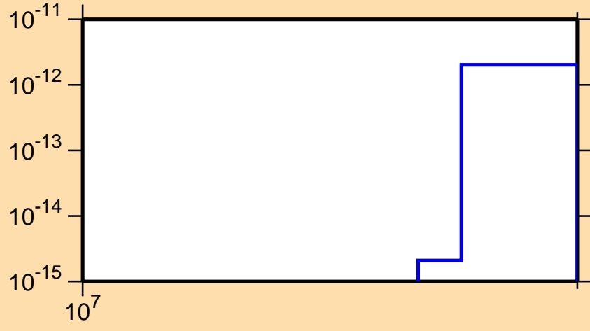
\sigma vs. E for ^{227}\text{Pa} (mt 11)
