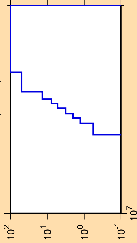
\Delta\sigma/\sigma vs. E for ^{227}\text{Pa}(\text{mt } 45)
