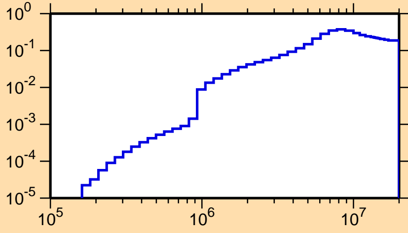
\sigma vs. E for ^{227}\text{Pa}(n,n\text{cont.})
