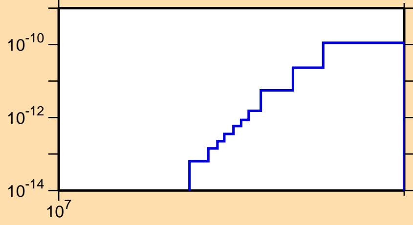
\sigma vs. E for ^{227}\text{Pa}(\text{mt } 45)
