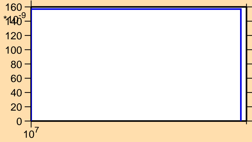
\sigma vs. E for ^{227}\text{Pa}(n,nt)
