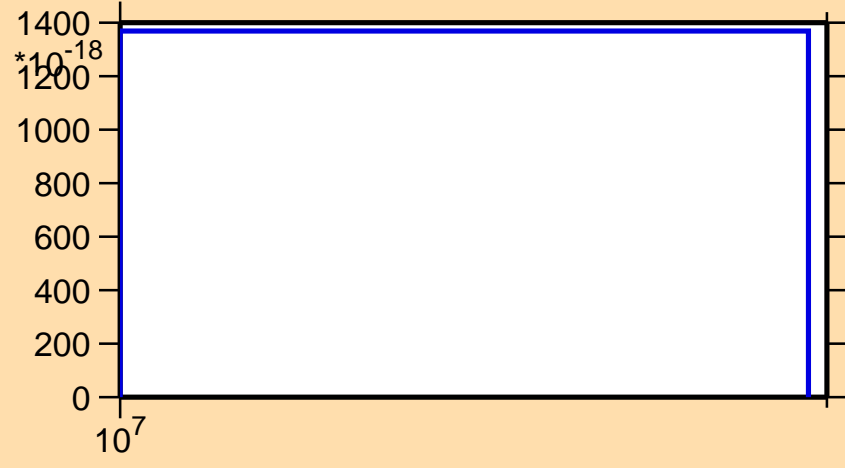
\sigma vs. E for ^{227}\text{Pa} (mt 42)
