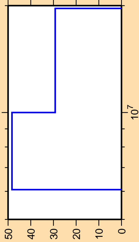
\Delta\sigma/\sigma vs. E for ^{227}\text{Pa}(n,t)
