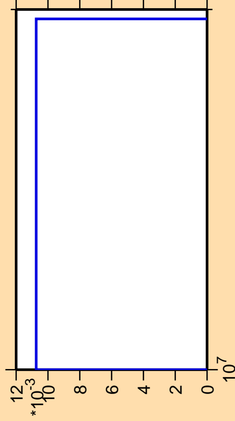
\Delta\sigma/\sigma vs. E for ^{227}\text{Pa} (mt 11)
