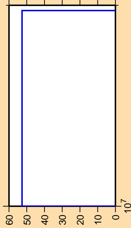
\Delta\sigma/\sigma vs. E for ^{227}\text{Pa}(\text{mt117})
