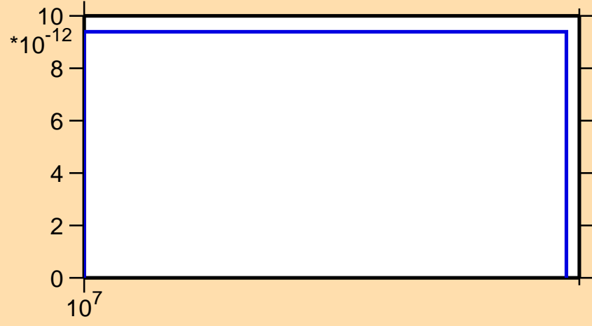
\sigma vs. E for ^{227}\text{Pa}(\text{mt117})
