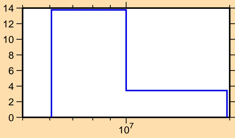
\Delta\sigma/\sigma vs. E for ^{227}\text{Pa}(n,\text{el.})
