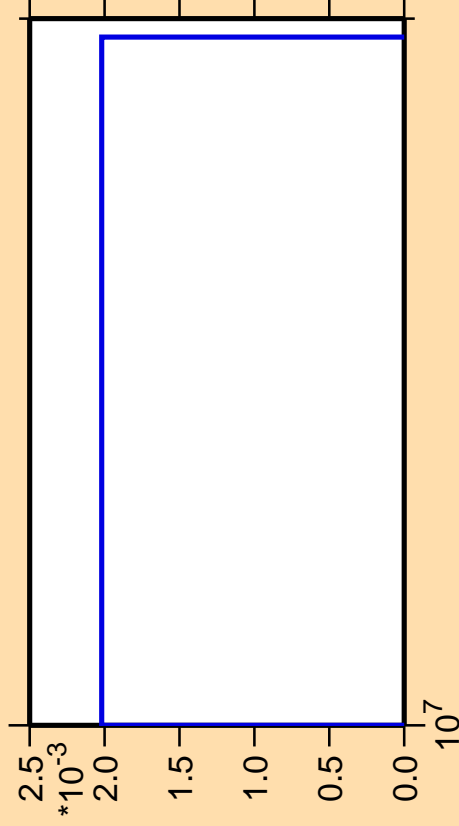
\Delta\sigma/\sigma vs. E for ^{227}\text{Pa} (mt 42)
