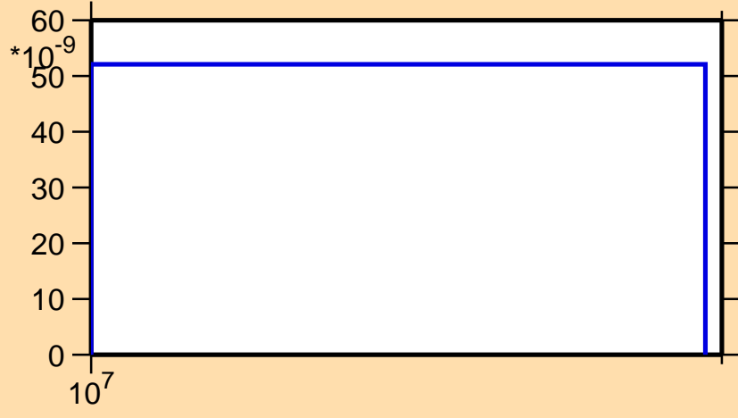
\sigma vs. E for ^{227}\text{Pa}(n,2np)
