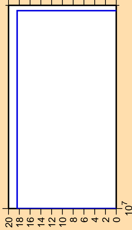
\Delta\sigma/\sigma vs. E for ^{227}\text{Pa} (mt 45)
