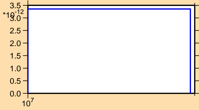
\sigma vs. E for ^{227}\text{Pa} (mt 45)
