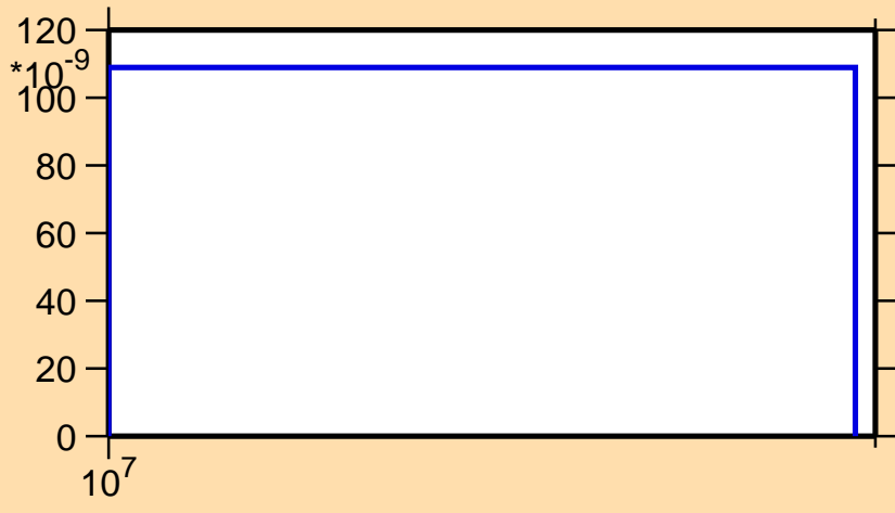
\sigma vs. E for ^{227}\text{Pa}(n,\text{nd})
