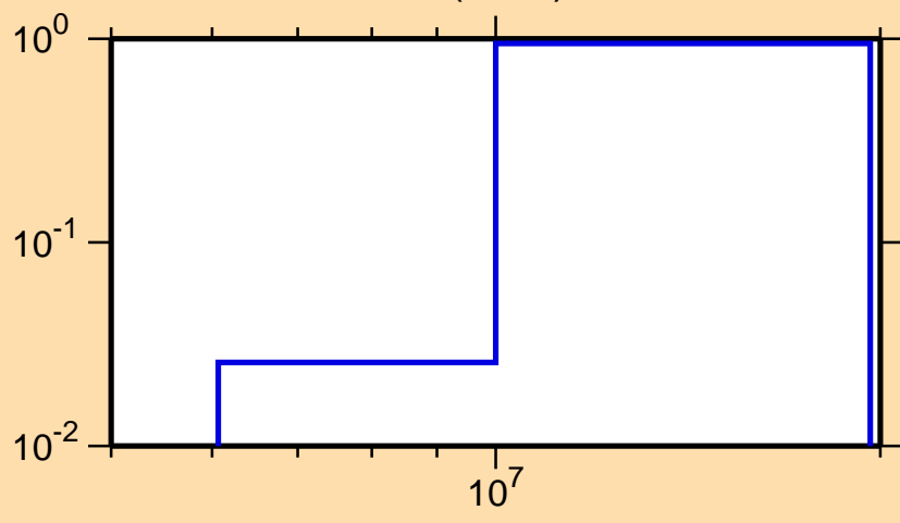
\sigma vs. E for ^{227}\text{Pa}(n,2n)
