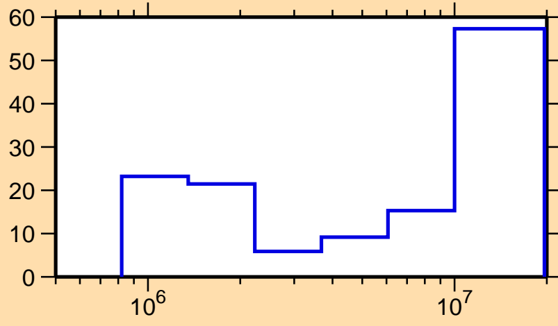
\Delta\sigma/\sigma vs. E for ^{227}\text{Pa}(n,f)
