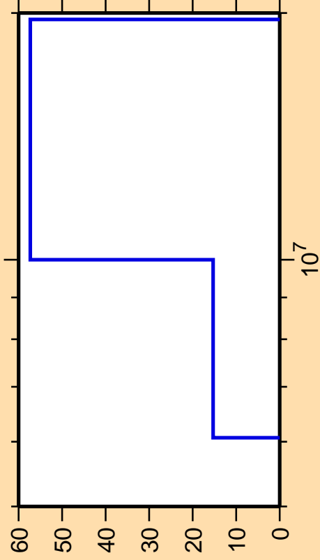
\Delta\sigma/\sigma vs. E for ^{227}\text{Pa}(n,f)
