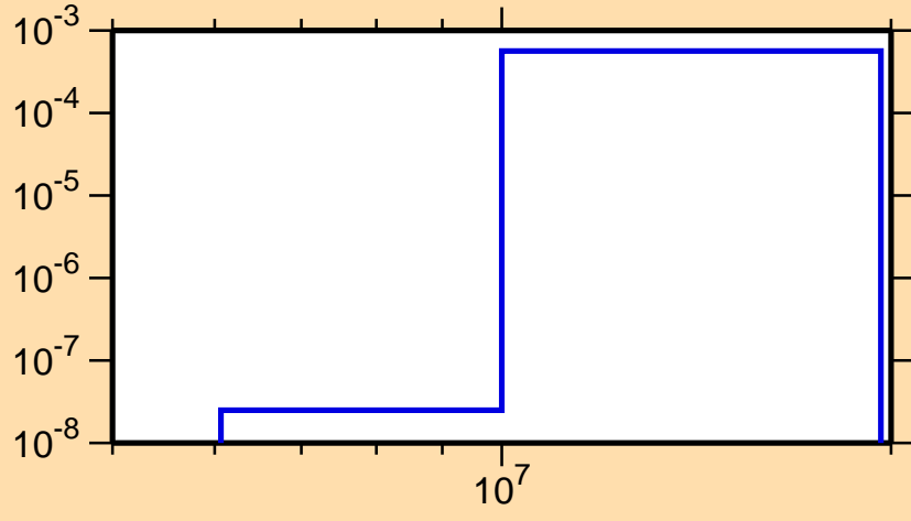
\sigma vs. E for ^{227}\text{Pa}(n,np)
