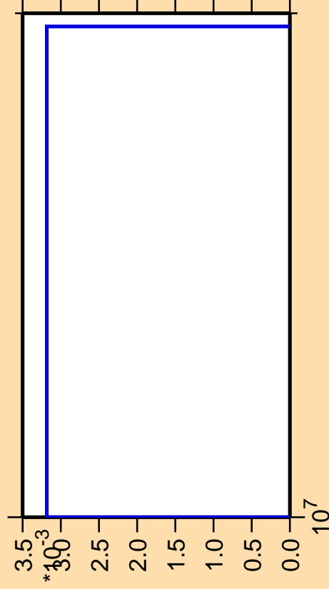
\Delta\sigma/\sigma vs. E for ^{227}\text{Pa} (mt 34)
