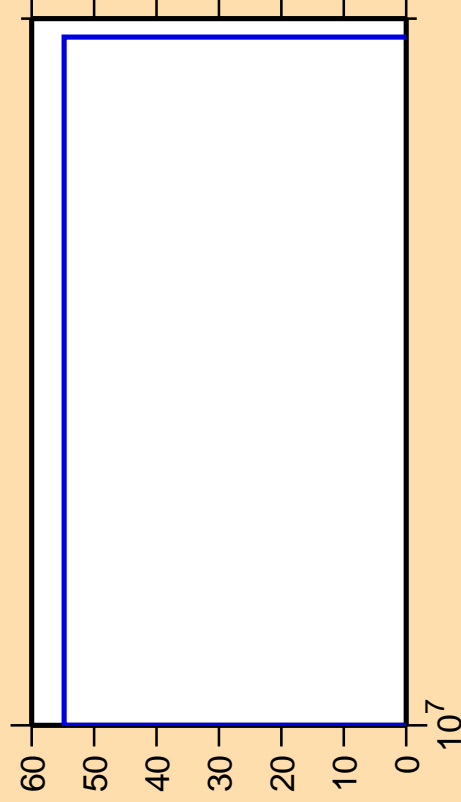
\Delta\sigma/\sigma vs. E for ^{227}\text{Pa}(n,nt)
