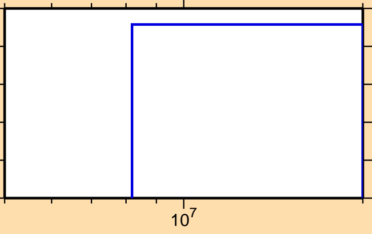
\sigma vs. E for ^{227}\text{Pa}(n,\text{nd})
