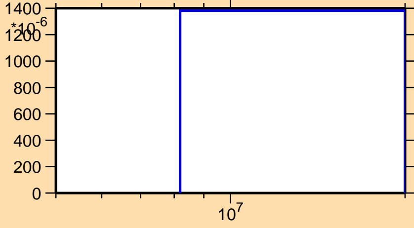
\sigma vs. E for ^{227}\text{Pa}(n,3n\alpha)
