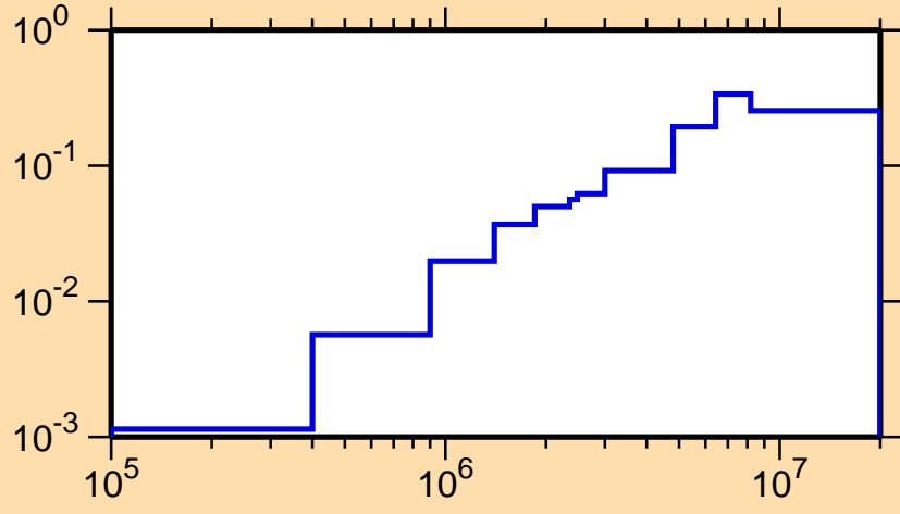
\sigma vs. E for ^{227}\text{Pa}(n,\text{inel.})
