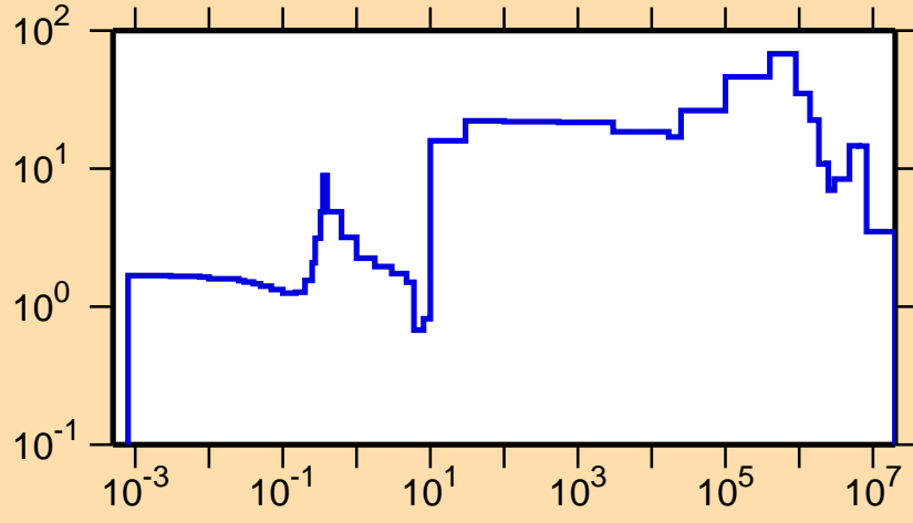
\Delta\sigma/\sigma vs. E for ^{227}\text{Pa}(n,el.)
