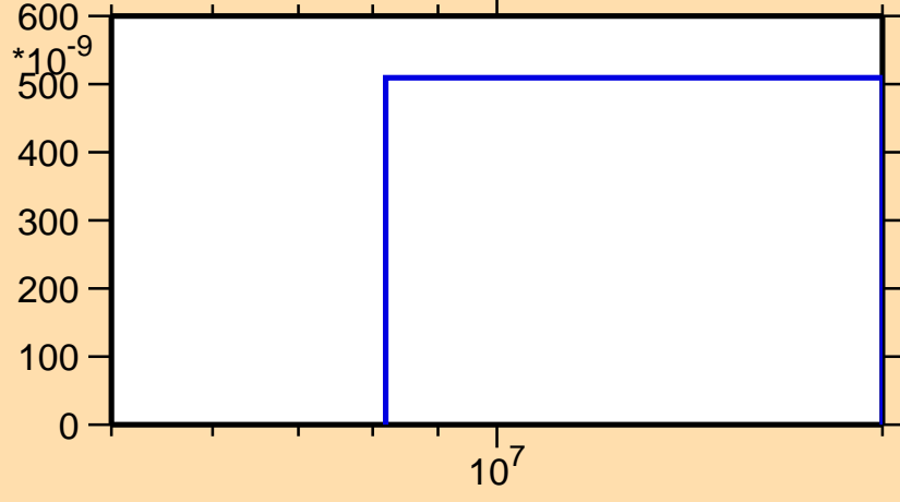
\sigma vs. E for ^{227}\text{Pa}(n,2n\alpha)
