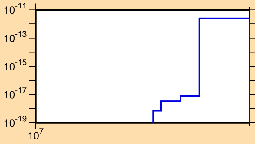
\sigma vs. E for ^{228}\text{Pa} (mt 11)
