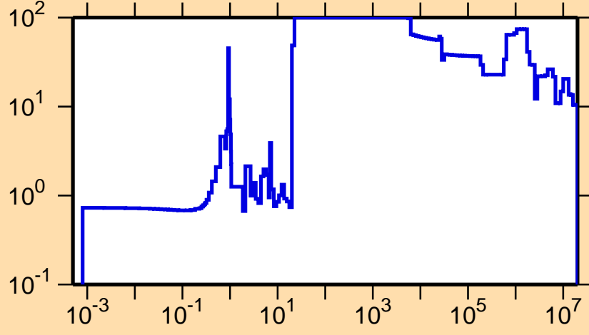
\Delta\sigma/\sigma vs. E for ^{228}\text{Pa}(n,el.)
