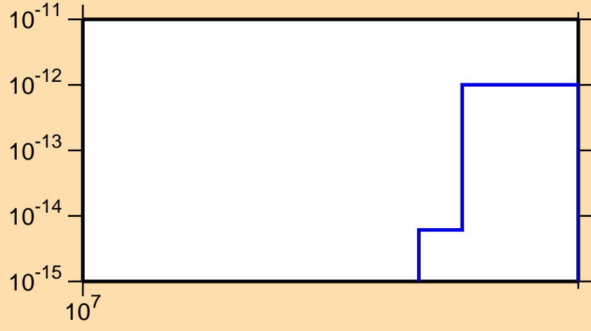
\sigma vs. E for ^{228}\text{Pa} (mt 34)
