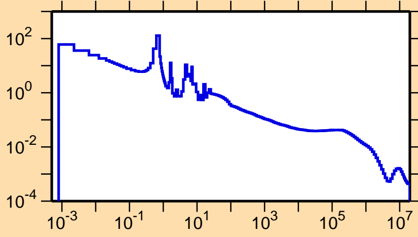
\sigma vs. E for ^{228}\text{Pa}(n,\gamma)
