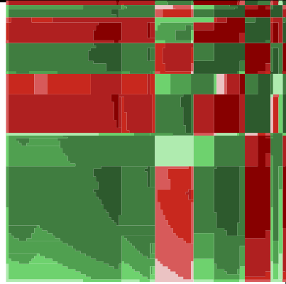
Correlation Matrix
