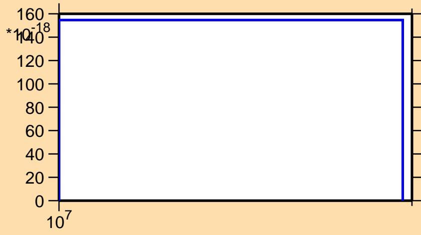
\sigma vs. E for ^{228}\text{Pa} (mt 42)
